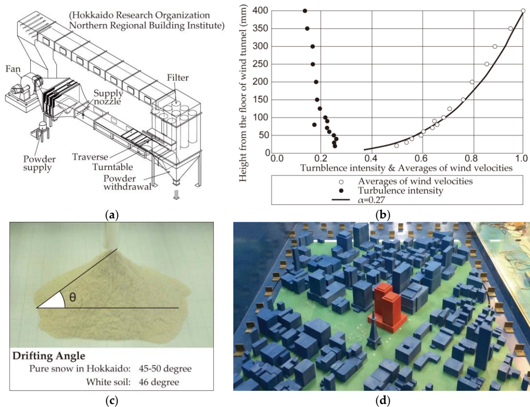
Figure 2. Snow simulation settings. (a) Wind tunnel; (b) Wind flow in experiments; (c) Activated clay (Snow model); (d) Simulation model.
