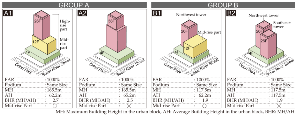
Figure 8. High-rise and high-density urban blocks in downtown Sapporo.
