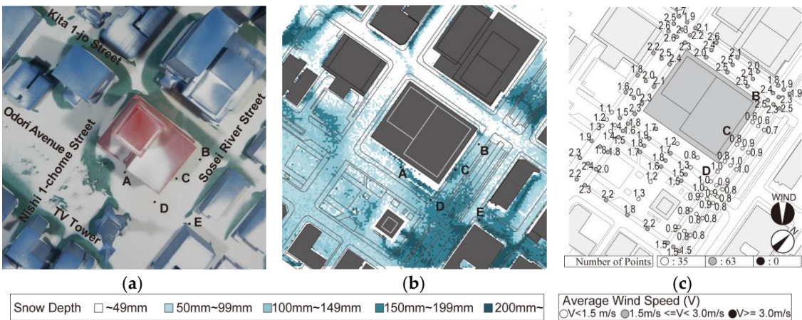
Figure 12. Snow and wind simulation results in Case B1. (a) Snow simulation result; (b) Snow depth; (c) Wind simulation result.
