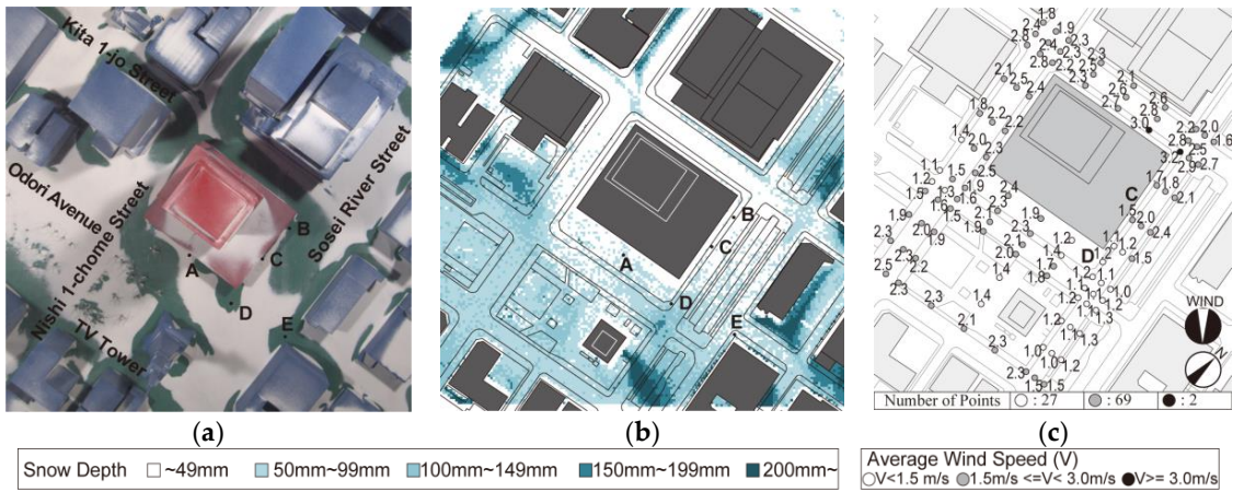
Figure 11. Snow and wind simulation results in Case A2. (a) Snow simulation result; (b) Snow depth; (c) Wind simulation result.
