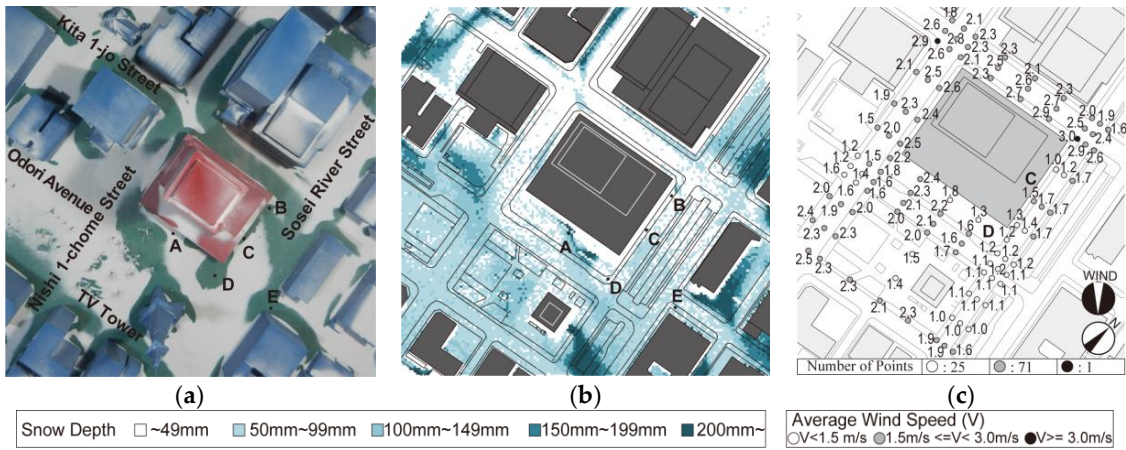
Figure 10. Snow and wind simulation results in Case A1. (a) Snow simulation result; (b) Snow depth; (c) Wind simulation result.
