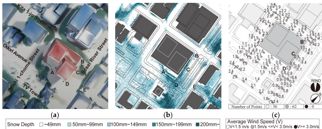
Figure 13. Snow and wind simulation results in Case B2. (a) Snow simulation result; (b) Snow depth; (c) Wind simulation result.
