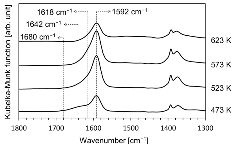
Figure 7. DRIFT spectra of Au-DP at different temperatures under a gas flow of H 2 and CO 2 .
