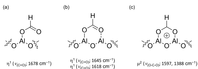
Figure 3. Proposed structures of adsorbed formate species on \text{Al}_2\text{O}_3 : (a) typical \eta^1 -type species, (b) two \eta^1 -type species interacting with weak and medium Lewis acid sites and (c) typical \mu^2 -type species.
