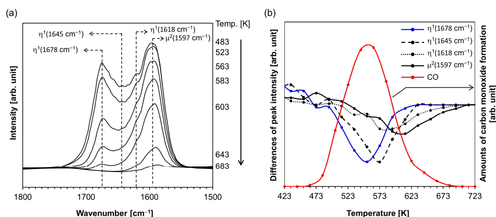
Figure 4. (a) DRIFT spectra of HCOOH-adsorbed Al 2 O 3 at different temperatures and (b) temperature dependence of CO formation and band intensities for four formates.
