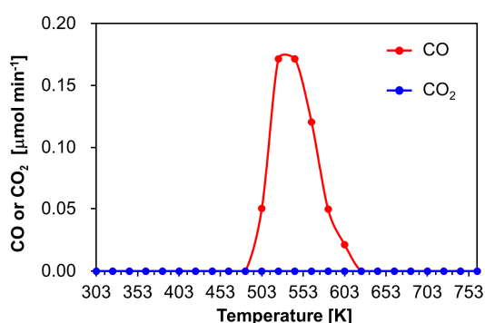
Figure 1. Dependence of CO (red) and CO 2 (blue) formation on reaction temperature over Al 2 O 3 .
