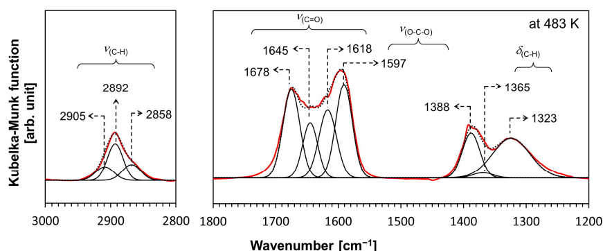
Figure 2. DRIFT spectrum of HCOOH-adsorbed Al 2 O 3 at 483 K under inert gas atmosphere. Red line: raw spectrum, black dot line: combined spectrum of deconvoluted peaks.
