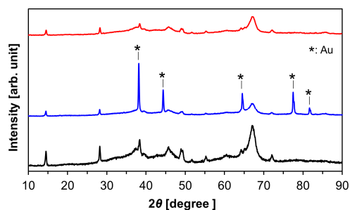
Figure 5. XRD patterns of \gamma -Al 2 O 3 (black), Au-Imp (blue) and Au-DP (red).
