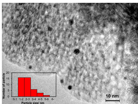
Figure 6. TEM image of Au-DP and size distribution of Au nanoparticles (inset).
