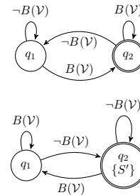
Fig. 4: DBA of L(\phi^{fair}) (top) and DMA of L(\phi^{cfair}) (bottom).
