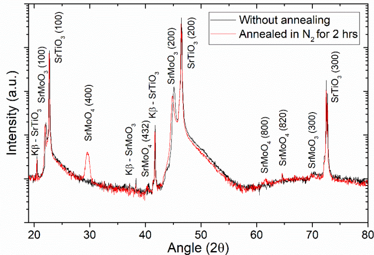
Fig. 1. XRD patterns for strontium molybdate samples produced with and without annealing in nitrogen.
