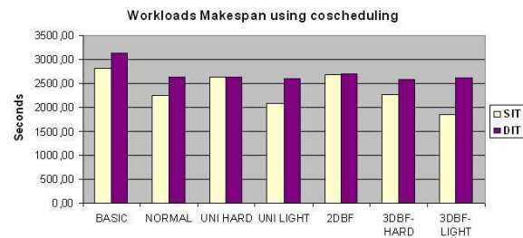
Figure 9 Workloads Makespan.
