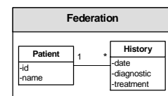
Figure 4: Case Study Federated Schema
