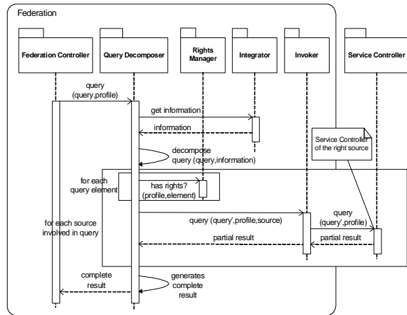
Figure 11: Query Interaction (Federation side)
