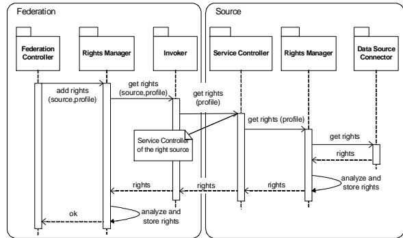
Figure 9: Rights Exportation Interaction
