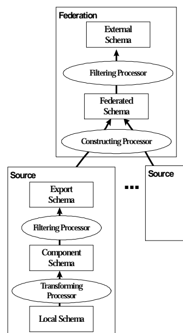
Figure 1: Five-level Architecture for Federated Systems
