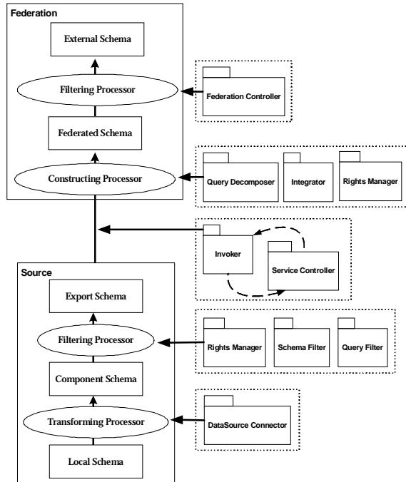
Figure 8: Designed Architecture - Five-level Architecture Mapping
