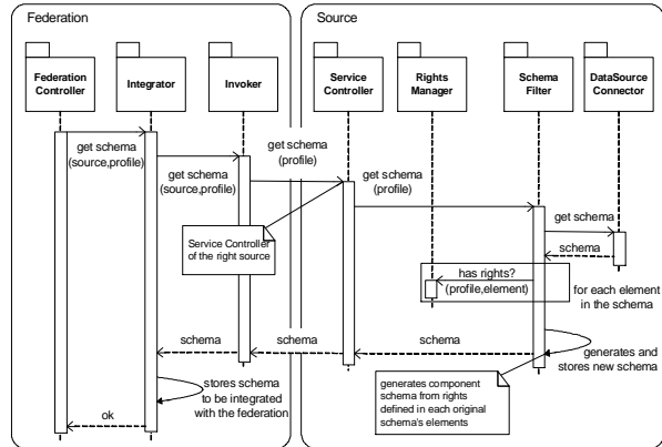
Figure 10: Schema Exportation Interaction
