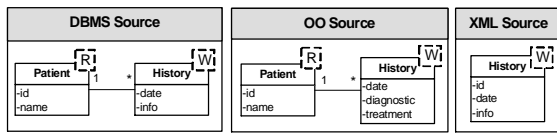
Figure 5: Export Schemas with Access Rights (R-Read, W-Write)
