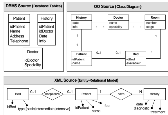
Figure 2: Case Study Sources
