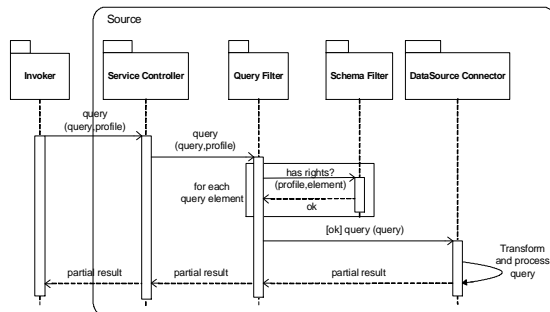
Figure 12: Query Interaction (Source side)
