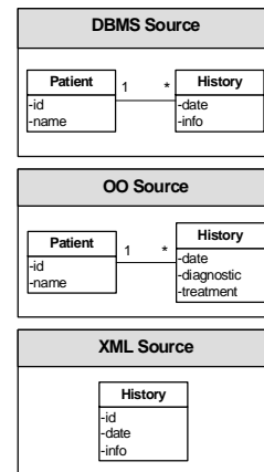
Figure 3: Case Study Export Schemas
