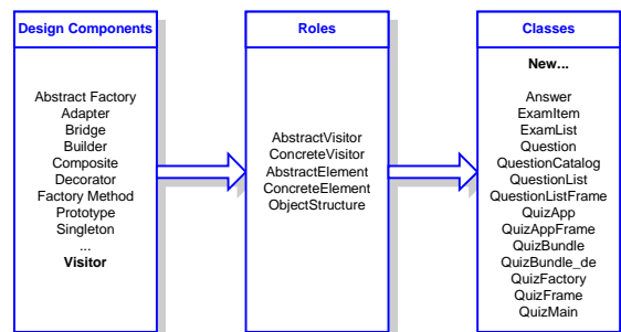
Figure 6-2: Instantiation Process
