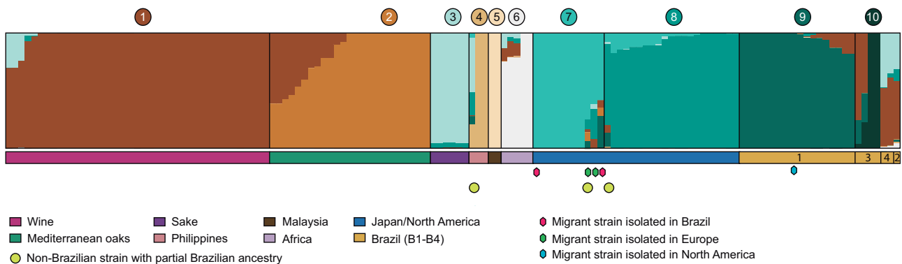
Fig. 4. —Population structure of S. cerevisiae . STRUCTURE plot based on a subset of 9,860 parsimony informative sites for K = 10 . Numbers from 1 to 10 represent the different clusters that capture the maximum representation of population ancestry. The phylogenetic groups inferred in figure 1 are “color-coded” at the bottom of the plot. Migrant strains are marked with “colored diamonds”: “red” (isolated in Brazil), “green” (isolated in Europe), and “blue” (isolated in North America). “Yellow circles” depict non-Brazilian strains with partial Brazilian ancestry.
