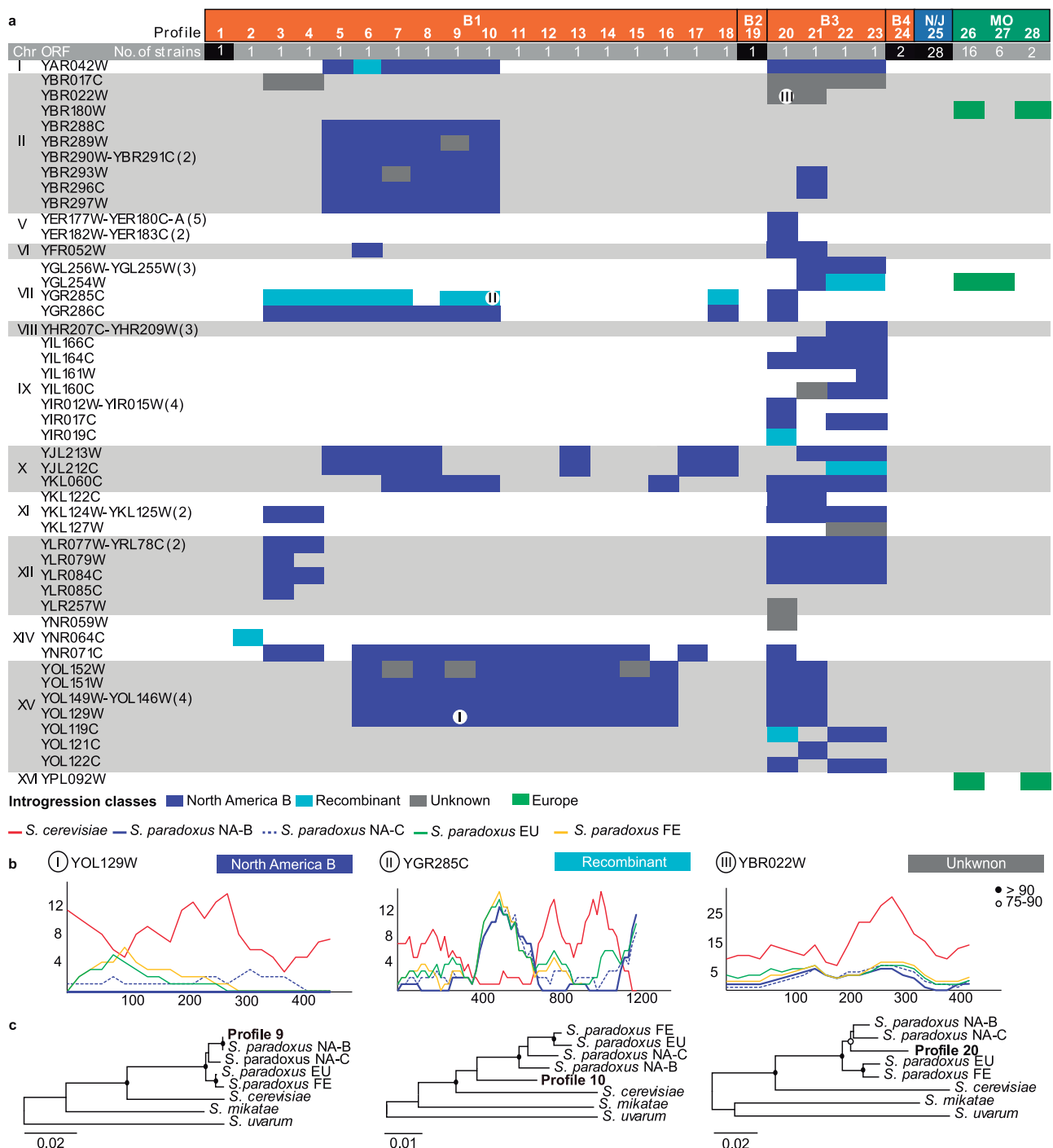
FIG. 6. —Introgressions of Saccharomyces paradoxus into S. cerevisiae . (a) Profiles of presence/absence of introgressions are numbered from 1 to 28 (profiles 1, 19, 24, and 25 depict absence of introgressions) and “color coded” according to the phylogenetic group (B—Brazil; N/J—North America/Japan; MO—Mediterranean oaks). The number of strains in each profile is depicted in the “gray bar” (numerals in “black boxes” refer to the number of strains without introgressions). The introgressed ORFs are listed on the “left side” and the four classes of introgressions are “color coded” (“dark blue”: S. paradoxus North American population B; “light blue”: recombinant S. cerevisiae × S. paradoxus North American population B; “gray”: S. paradoxus —unknown population; and “green”: S. paradoxus —European population). (b) Divergence plots of exemplary sequences showing cases of ORFs introgressed from S. paradoxus North American population B (I); recombinant S. cerevisiae × S. paradoxus North American population B (II); and unknown population of S. paradoxus (III). (c) Phylogeny of introgressed ORFs (same ORFs as in b), using for comparison the available sequences from the different populations of S. paradoxus , and the orthologs of S. cerevisiae , S. mikatae , and S. uvarum .
