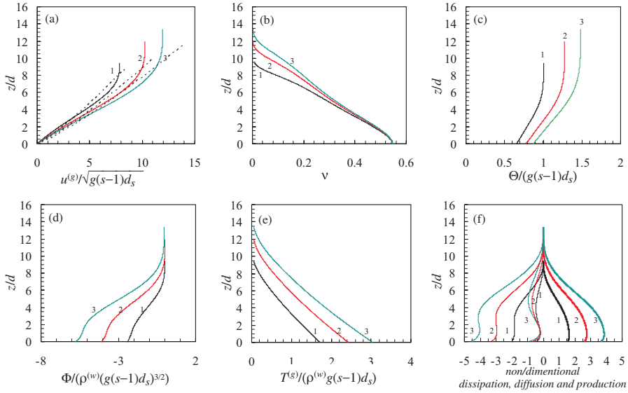
Figure 3. Computed profiles of non-dimensional quantities in the transport layer. Simulations 1, 2 and 3 correspond to, respectively, \theta = 1.74, \theta = 2.49 and \theta = 3.07 .
