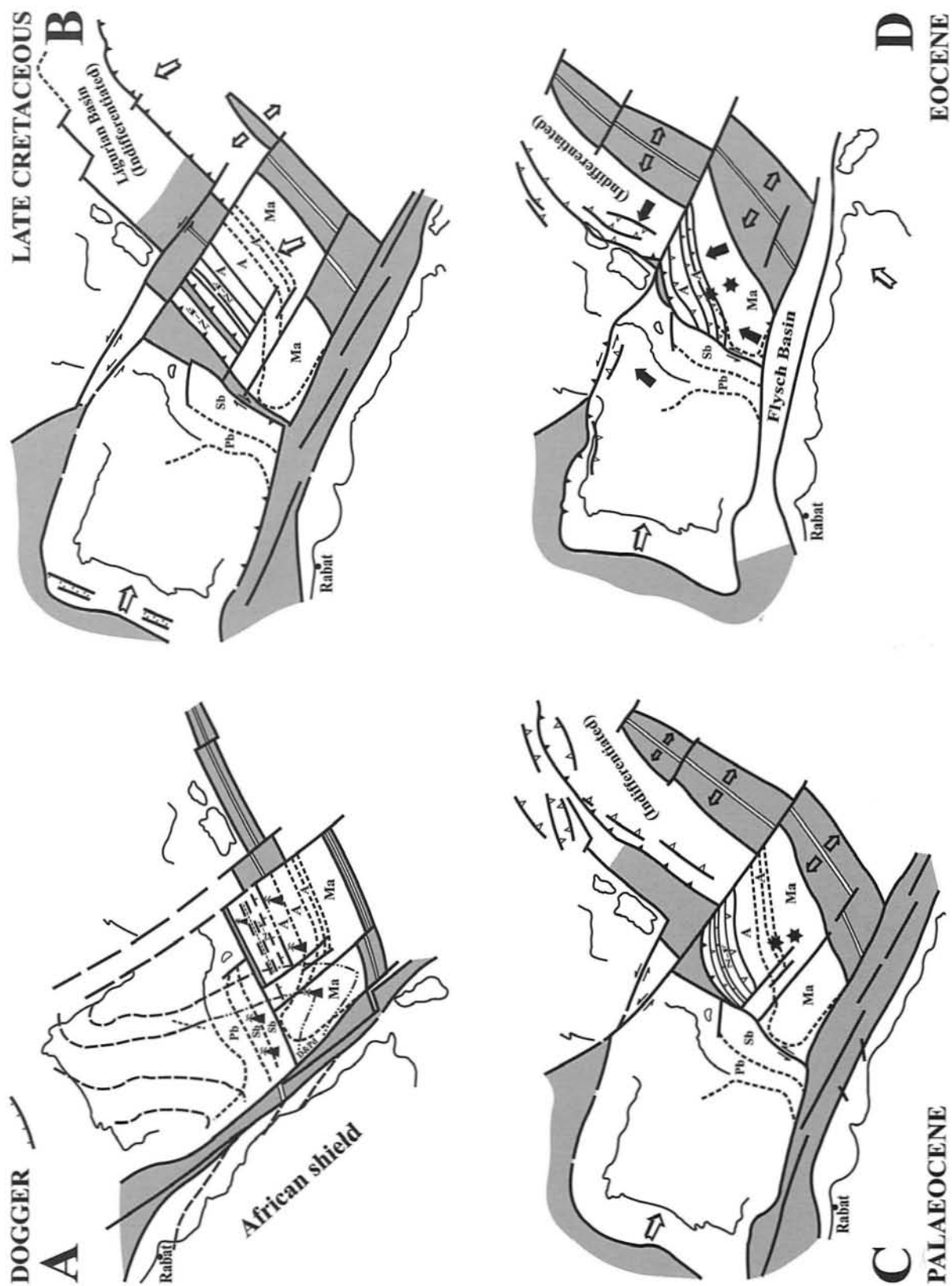
Fig. 3 - Interpretative schemes of the evolution of Iberia. A: Situation of Iberia at the beginning of the Dogger, when the western Mediterranean area was affected by extension. B: During the Late Cretaceous, the western Mediterranean, after the rotation of Iberia, underwent the first compressions. C: During the Palaeocene, the process of subduction of the western Mediterranean affected strongly the Betic Internal Zone. D: During the Eocene, the Pyrenees, Cantabrian area and the Betic Internal Zone underwent important compressions. Key of the abbreviations: A: Alpujarride, D & Pd: Dorsal and Predorsal, Ma: Malaguide, N-F: Nevado-Filabride, Pb: Prebetic, Sb: Subbetic. Taken from Sanz de Galdeano (1997). The arrows indicate the direction of tectonic transport. Opposed arrows: extension. Stars: peridotite intrusions. Grey colours: oceanic crust.
