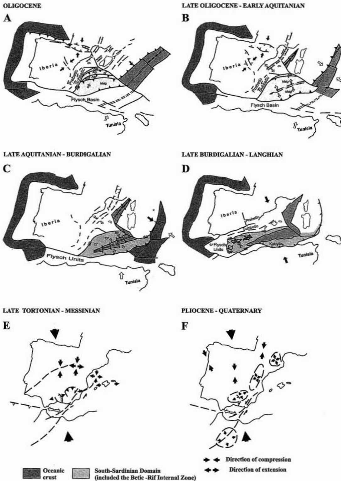
Fig. 6 - Interpretative schemes of the evolution of SE Iberia. A: During the Oligocene, continued the deformations in the Pyrenees and in the Betic-Internal Zone and began the structuration of the Iberian Cordillera. B: During the Late Oligocene- Early Miocene, the opening of the Algero-Provençal basin accelerated. Then began the overthrusting of the Malaguide Complex over the Alpujarride and, immediately, the extension of the Algerian Basin prolonged to the Alboran area. C: During the Early Miocene continued the opening of the Algerian Basin and, especially, during the Burdigalian the Betic-Rif Internal Zone was westwards expelled. D: This westwards expulsion continued during the Late Burdigalian till the Middle Miocene. The Flysch Basin and the Subbetic were strongly deformed. E: During the Late Miocene, N-S to NNW-SSE compressions affected the entire Iberia, combined in many points with a near E-W extension. F: Continued the same geodynamic situation, but some eastern areas of Iberia underwent radial extension. Alp: Alpujarride; Malg: Malaguide. A to D taken from Sanz de Galdeano (1997).
