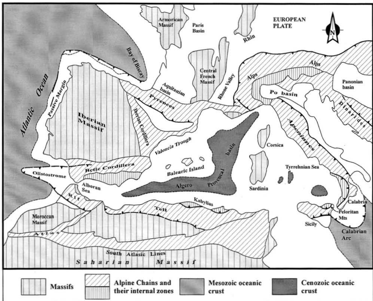
Fig. 1 - Geological situation of Iberia.
