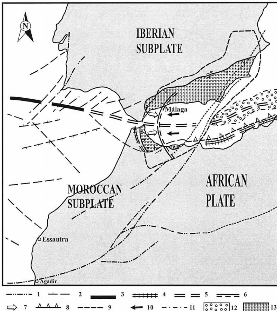
Fig. 8 - Interpretation of the present tectonic situation of the Iberian-Moroccan area. 1: Faults. 2: Probable faults. 3: Approximate contact between the Iberian and African plates. 4: Former contact between the African plate and the South-Sardinian domain. 5: Possible prolongation to the east of the contact between the African and Iberian plates. 6: Position of the arc produced by the sinking of the Iberian and African lithospheres in the W Alboran Sea. 7: Arrows indicating direction of crustal sinking in the W Alboran Sea. 8: Present boundary of the Betic-Rif Internal Zone. 9: Position, according Blanco & Spackman (1993) of the sunken lithospheric sheet in the Betic-Rif area. 10: General direction of displacement of the Betic-Rif Internal Zone. 11: Approximate limit of the oceanic crust. 12: Oceanic crust in the Algerine Basin. 13: Betic-Rifain internal zone.
