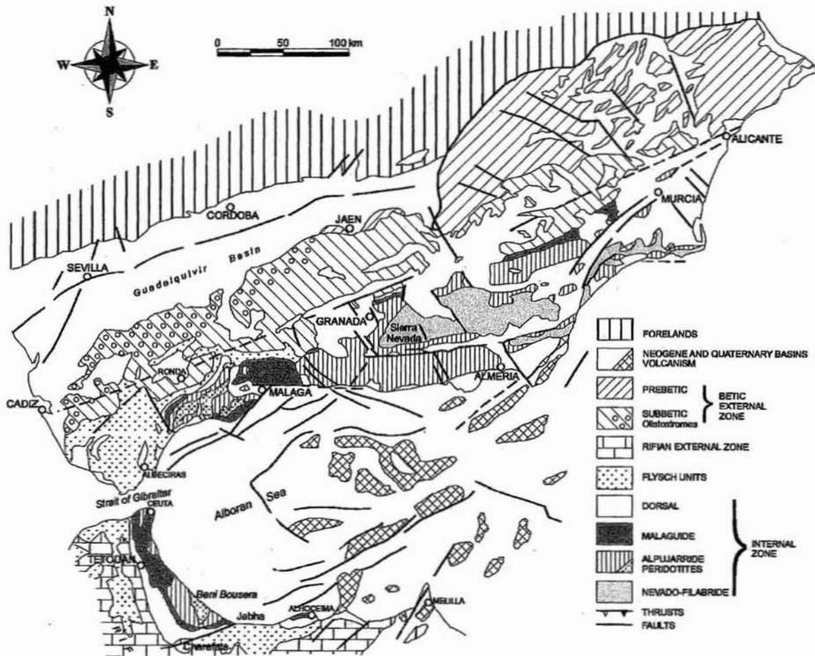
Fig. 4 - General geologic map of the Betic Cordillera.
