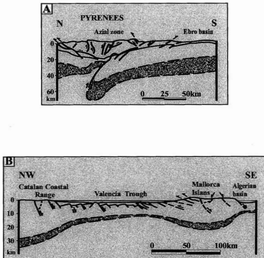
Fig. 5 - Schematic geological cross-sections. A: Interpretation of the geological structure of the Pyrenees. Simplified from Muñoz (1992) and modifications inspired in Velasque et al. , (1989). B: Structure of the Valencia trough. Simplified from Martí et al. (1992) and Fontboté et al. (1990). Lower crust in points. Their position is marked in Fig. 2.
