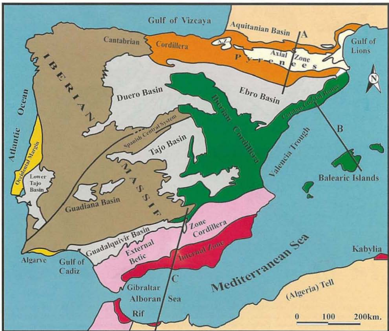
Fig. 2 - Highly simplified geological scheme of the principal domains in the Iberian Peninsula (simplified and modified from Julivert et al. , 1972). The position of cross-sections of figures 5 and 7 is marked.
