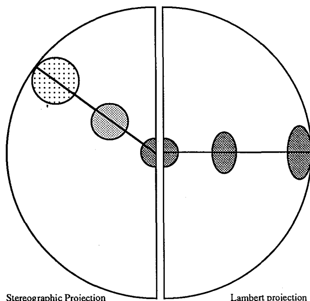
Fig. 6 — Comparison between the deformations induced by the stereographic and the Lambert projections.
