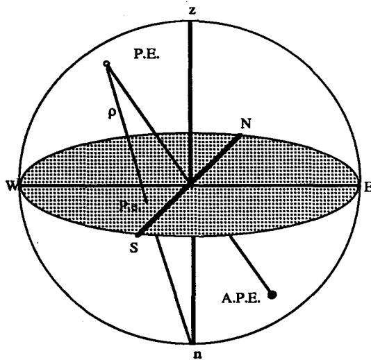
Fig. 1 — Stereographic Projection (perspective of the Miller sphere). z - zenith; n - nadir; P.E. - spheric pole; A.P.E. - spheric antipole; P.e. - stereographic pole; \rho - projectant ray.
