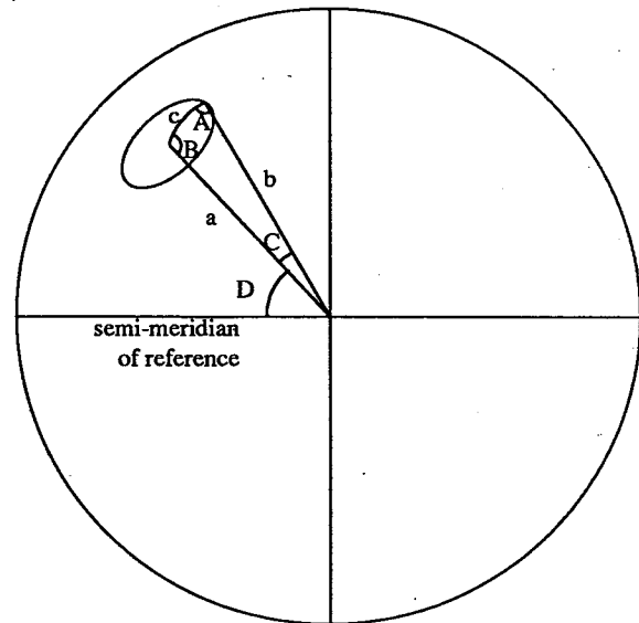
Fig. 9 — Drawing of small circles by calculating the coordinates of all its points.
