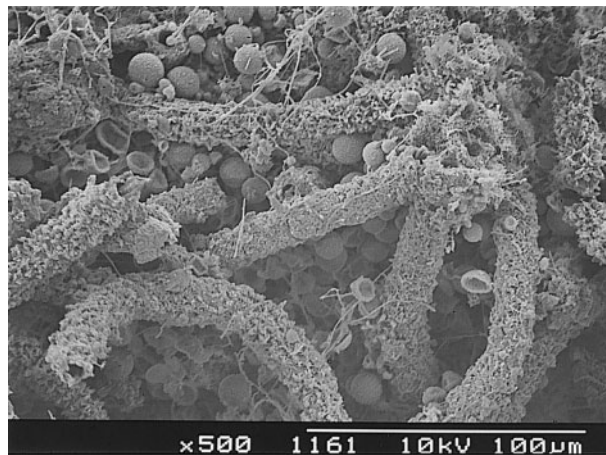
Fig. 10. SEM micrograph of Scytonema julianum mat. The calcified sheaths are composed of triradial calcite crystals. Scale bar, 100 µm. Reproduced from Ortega-Calvo et al. (1995) with permission.
