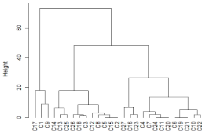
Figure 3.1.8 - Cluster Dendrogram
