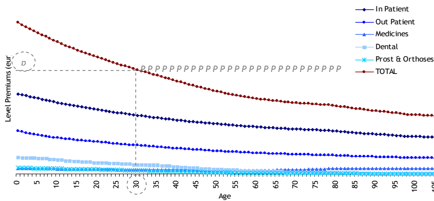
Figure 3.1.5 - Pure Level Premium to whole life health insurance
