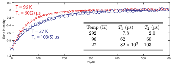
FIG. 5. T_2 decoherence lifetimes measured by echo decay at 96 and 27 K in sample B. Inset: comparison of T_1 and T_2 spin-lifetimes. The measured T_2 is effectively limited by T_2 \leq 2T_1 at room temperature and 96 K, but has reached a non- T_1 -limited value of 103 \mu\text{s} at 27 K.
