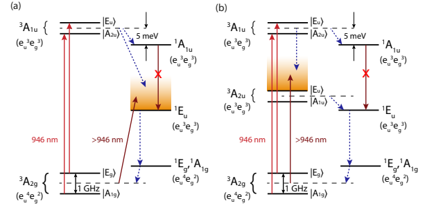
FIG. 6. Possible mechanisms for generation of spin polarization into the GS m_s = 0 state based on intersystem crossing (ISC) within \text{SiV}^0 . Optical transitions are given as solid arrows; non-radiative transitions are dotted. The molecular orbital configuration for each state is given in brackets, spin-orbit (SO) states are given and spin-spin effects have been neglected. (a) Spin polarization occurs by spin-orbit coupling between the ES and a singlet state; below-ZPL polarization is generated by a dipole-allowed transition from the GS to the singlet which becomes weakly allowed due to SO mixing in the GS. (b) Spin polarization is generated by ISC from a third triplet state between the GS and ES. ZPL dipole transitions between the GS and the {}^3A_{2u} are forbidden, but can be driven into the vibronic sideband by emission of A_{2g} phonons. In both cases the given singlet characters are examples; however, there can be no dipole transition between singlets in order for the upper singlet to be an effective shelving state, as observed in temperature-dependent PL measurements [10]. In comparison to the well-understood model for \text{NV}^- [29], our model must also account for spin polarization at below-resonant energies.
