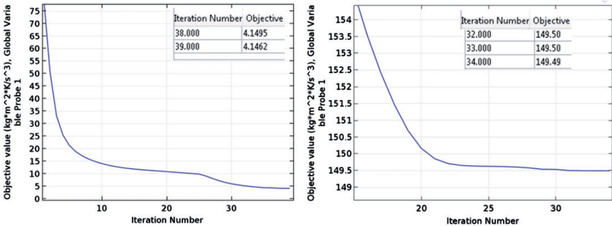
Figure 8. Convergence of Objective value for k_f/k_s=0.001 and k_f/k_s=0.1 .
