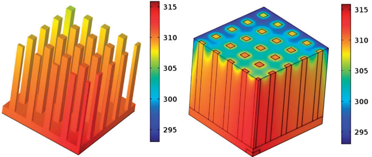
Figure 15. Temperature distribution from CFD study on Standard heat sink for k_f/k_s=0.001 .
