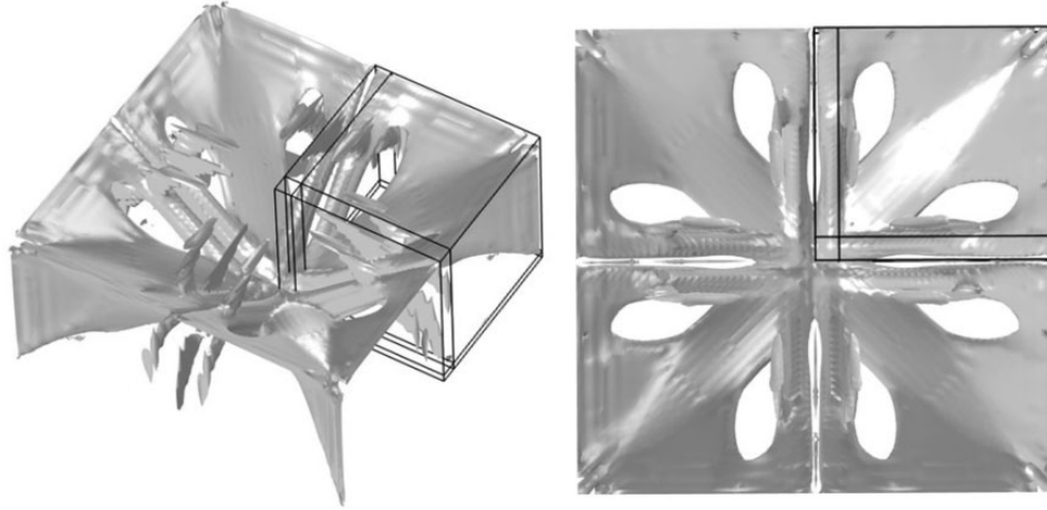
Figure 4. Full view of optimised heat sink (isometric, top view) by DM for k_f/k_s=0.001 .
