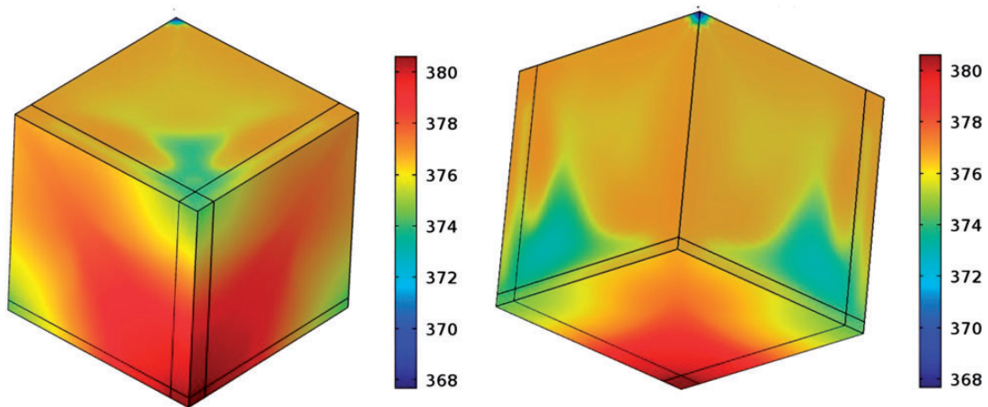
Figure 5. Temperature contour in the design domain for optimised heat sink by DM method for k_f/k_s=0.001 (top view & bottom view).
