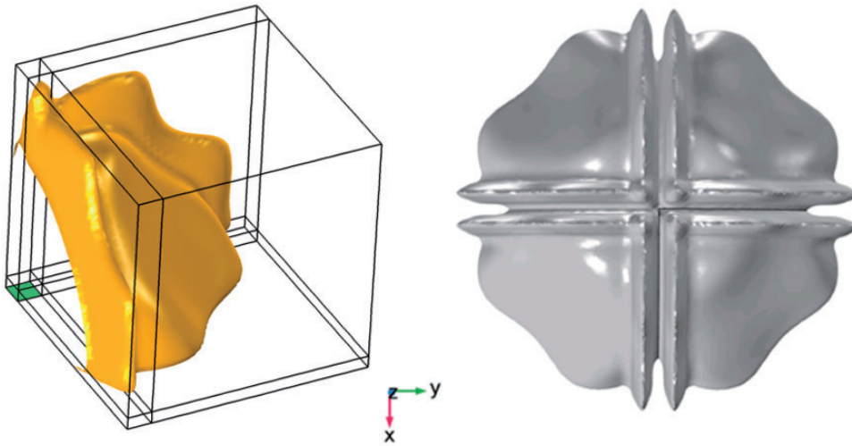
Figure 6. DM optimised heat sink for k_f/k_s=0.1 and its full symmetrised view.
