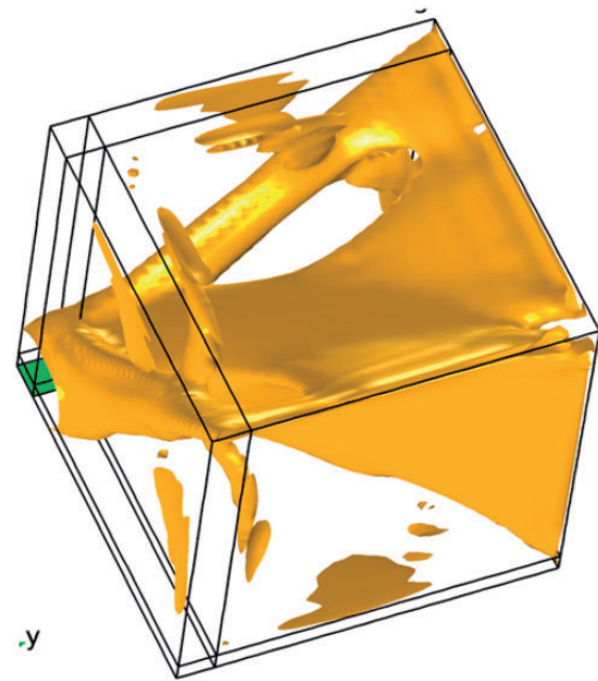
Figure 3. DM optimised heat sink for k_f/k_s=0.001 .
