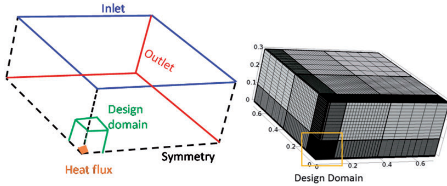
Figure 2. Computational domain of 3D heat sink design study.
