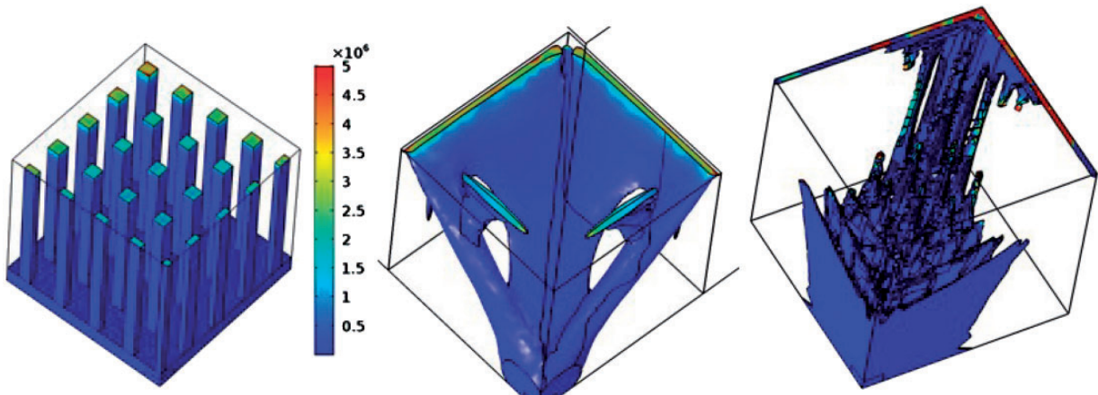
Figure 18. Temperature gradient comparison between Standard heat sink, DM & LSM heat sinks for k_f/k_s=0.001 .
