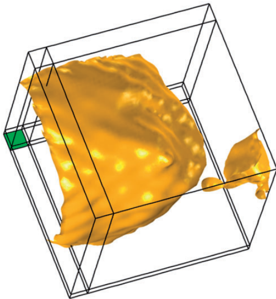
Figure 14. Optimised shape for k_f/k_s=0.1 through LSM with initialisation B.
