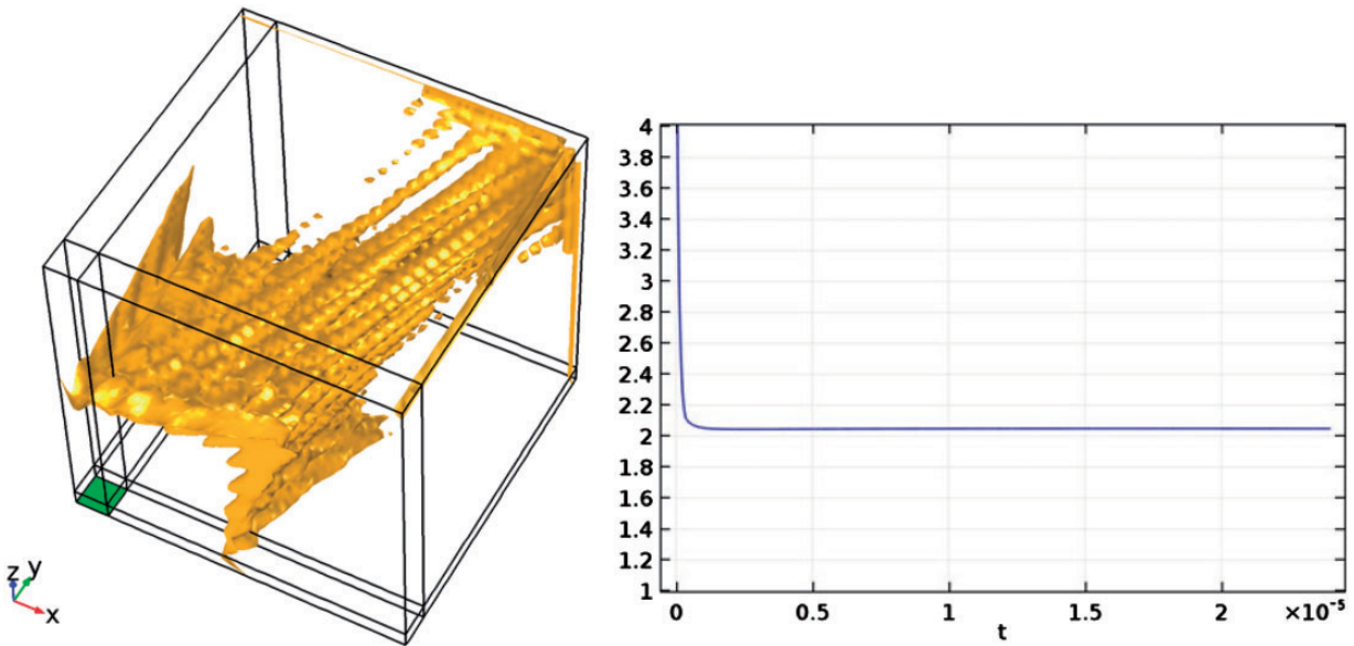
Figure 11. Optimised shape for k_f/k_s=0.001 through LSM with initialisation A and the convergence plot.
