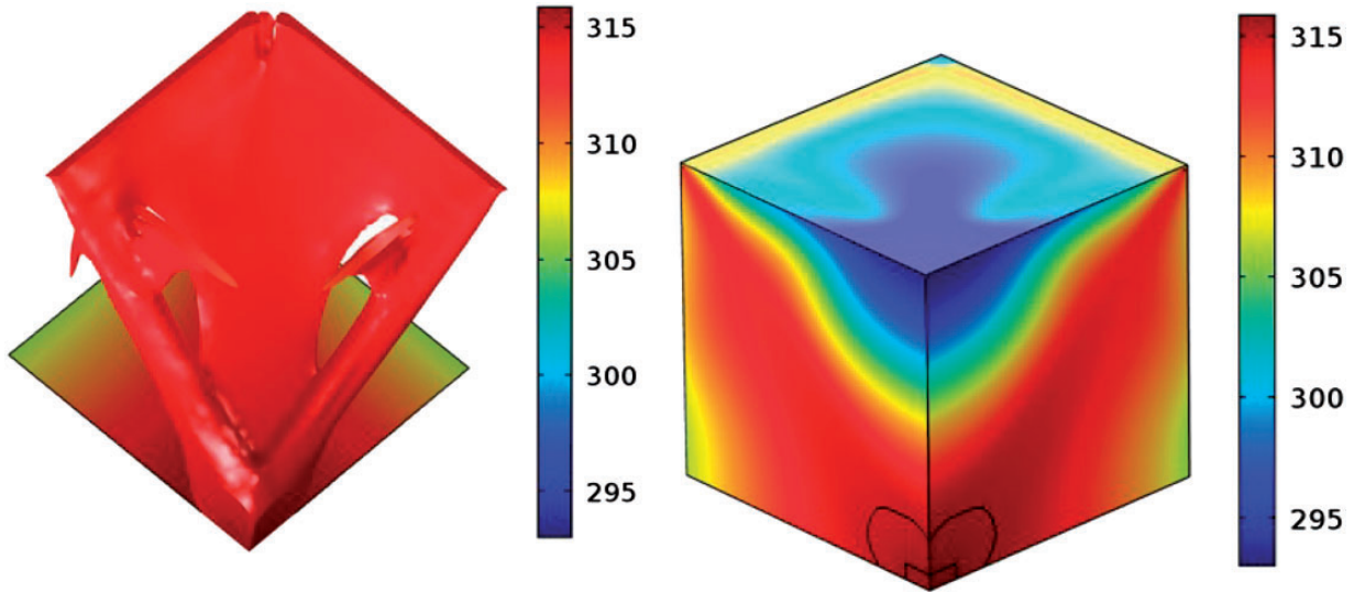
Figure 16. Temperature distribution from CFD study on DM heat sink for k_f/k_s=0.001 .
