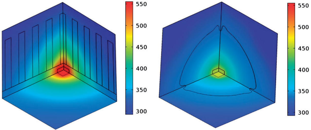
Figure 19. CFD-based temperature contours of Standard and DM heat sinks for k_f/k_s=0.1
