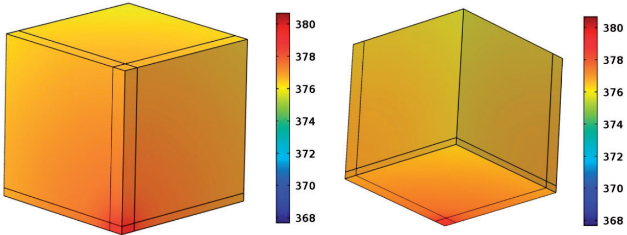
Figure 13. Temperature contour on design domain for optimised shape for k_f/k_s=0.001 through LSM with initialisation B.
