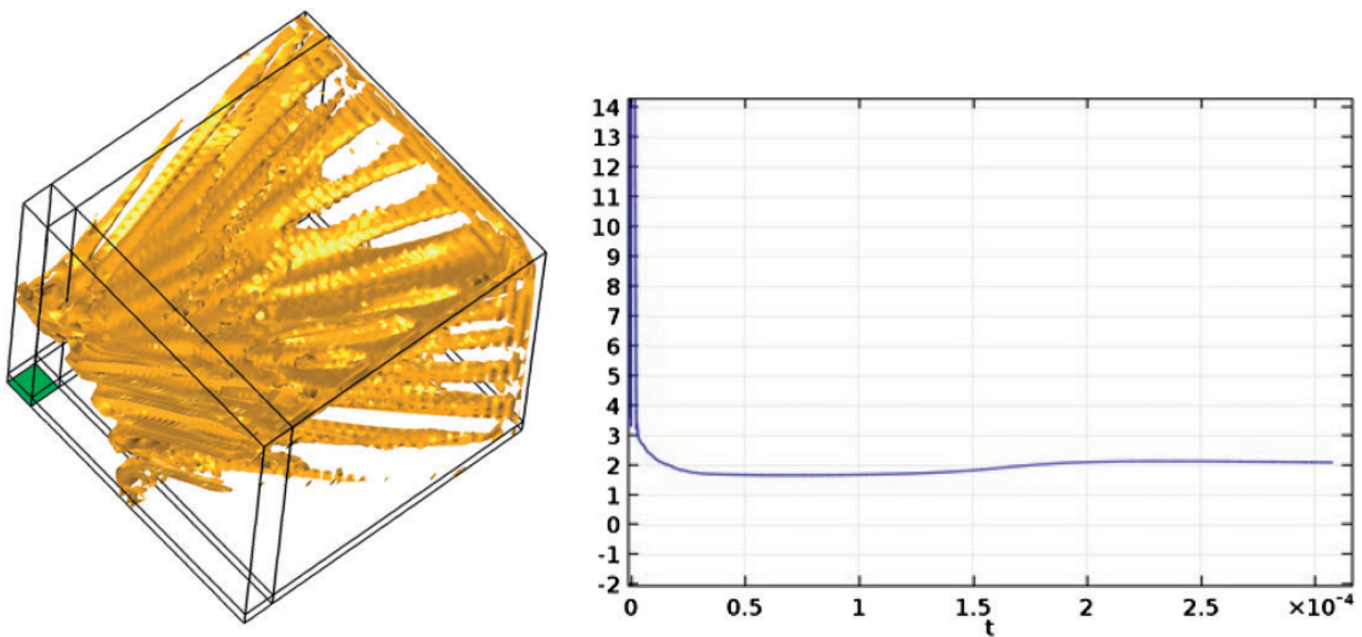
Figure 12. Optimised shape for k_f/k_s=0.001 through LSM with initialisation B.
