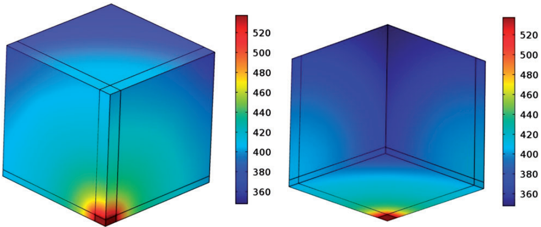
Figure 7. Temperature contour in the design domain for optimised heat sink by DM for k_f/k_s=0.1 (top & bottom view).
