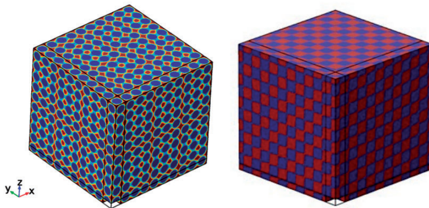
Figure 10. Initial Level set distributions uniform sphere (A) and cube distributions (B).
