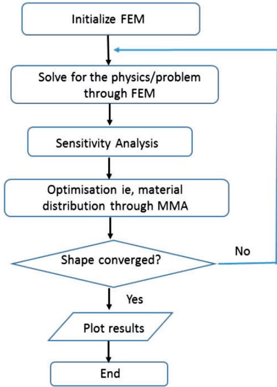
Figure 1. Flow chart illustrating DM procedure.
