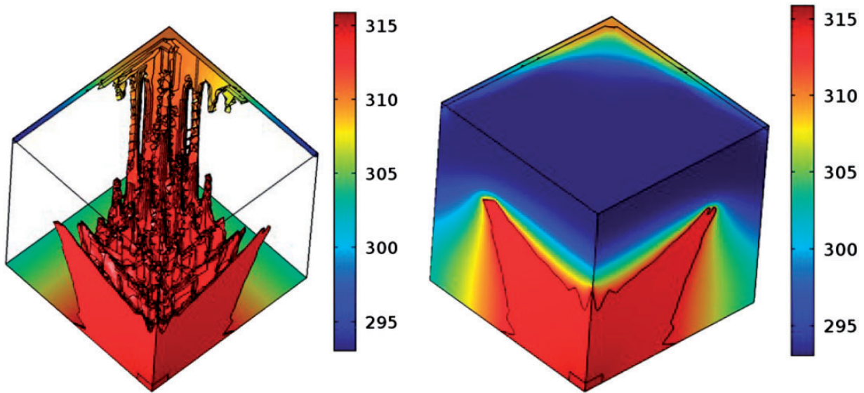
Figure 17. Temperature distribution from CFD study on LSM heat sink for k_f/k_s=0.001 .
