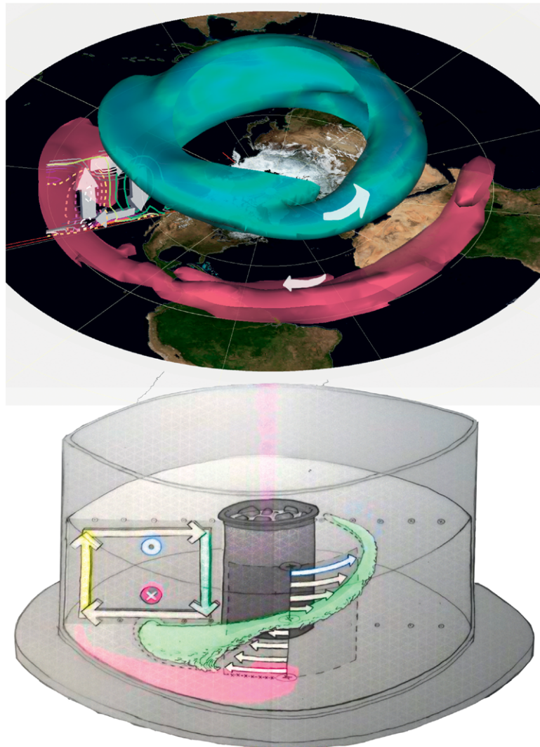
FIG. 6. (top) Climatological winter mean circulation, showing upper-level westerlies (cyan isosurface of u = 30 \text{ m s}^{-1} ) and low-level easterlies (pink isosurface of u = -10 \text{ m s}^{-1} ). The meridional section on the left-hand side shows the zonally averaged overturning circulation at low latitudes; vertical and meridional wind directions are marked by white arrows. (All fields are plotted using IDV software.) (bottom) A schematic diagram of the laboratory Hadley circulation, showing similar features to the observed climatology: the green streak of “westerlies” and the pink plume of “easterlies” (cf. with Fig. 5).
