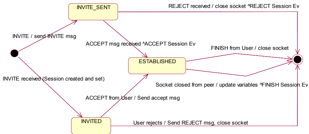
Figure 7 - Session States Diagram
