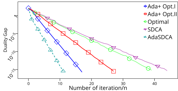
Figure 4. ijcnn1 dataset d = 22 , n = 49990 , Quadratic loss with L_2 regularizer, comparing number of iterations with known algorithms
