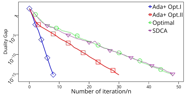
Figure 22. mushrooms dataset d = 112 , n = 8124 , Smooth Hinge loss with L_2 regularizer, comparing number of iterations with known algorithms
