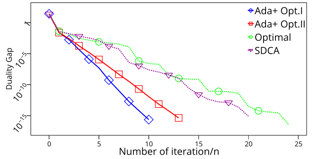
Figure 21. dorothea dataset d = 100000 , n = 800 , Smooth Hinge loss with L_2 regularizer, comparing number of iterations with known algorithms
