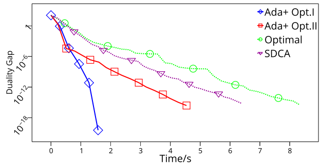
Figure 14. ijcnn1 dataset d = 22 , n = 49990 , Smooth Hinge loss with L_2 regularizer, comparing real time with known algorithms
