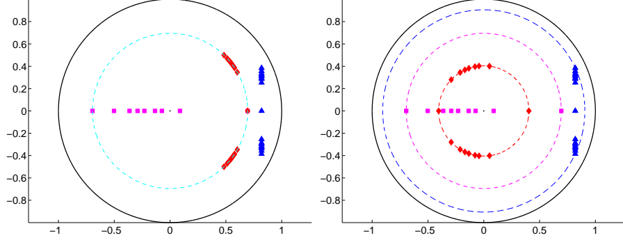
Figure 6: On the left, the spectrum of G_1(\theta_1^*) (magenta squares), G_2(\theta_2^*) (blue triangles) and G_3(\theta_1^*) (red diamonds). On the right, the spectrum of G_3(\theta_3^*) , where \theta_3^* is the optimal parameter.
