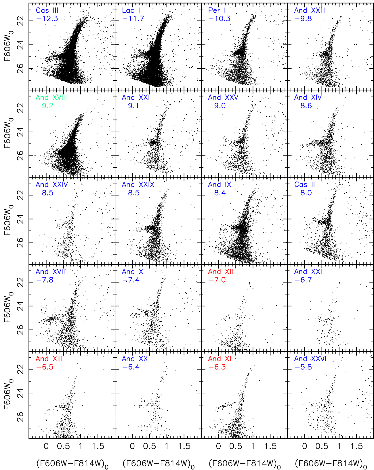
Figure 2. CMDs of the 20 dwarf galaxies in our sample, ordered by decreasing luminosity. Each CMD includes stars within the full ACS field or the region with 2r_h of that dwarf galaxy, whichever is smallest. The numbers listed in the top-left corner of each panel correspond to the M_V value of that system (Martin et al. 2013b, 2013c, 2016; Slater et al. 2015; Rhode et al. 2017). Systems with blue labels were observed in our program (HST-GO-13699), whereas systems with red labels were observed with WFPC2 as part of program HST-GO-11084. And XVIII, shown with a green label, was observed with ACS as part of the HST-SNAP-13442 program, which had similar observational properties. Note the predominance of red HBs overall.
