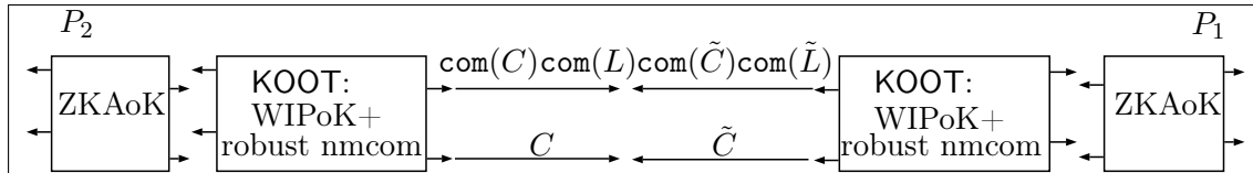
Figure 2: The 4-round protocol of [GMPP16b] for any functionality assuming 3-round 3-robust parallel non-malleable commitments in the simultaneous message exchange model.
