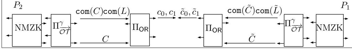
Figure 3: Our 4-round protocol for any functionality assuming trapdoor permutations in the simultaneous message exchange model. c_0 and c_1 ( \tilde{c}_0 and \tilde{c}_1 ) are commitments of P_2 's ( P_1 's) input.
