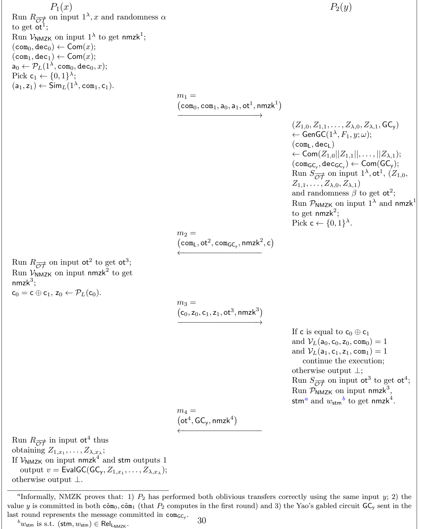
Figure 6: High-level description of the left execution of \Pi_{2\mathcal{PC}} .
