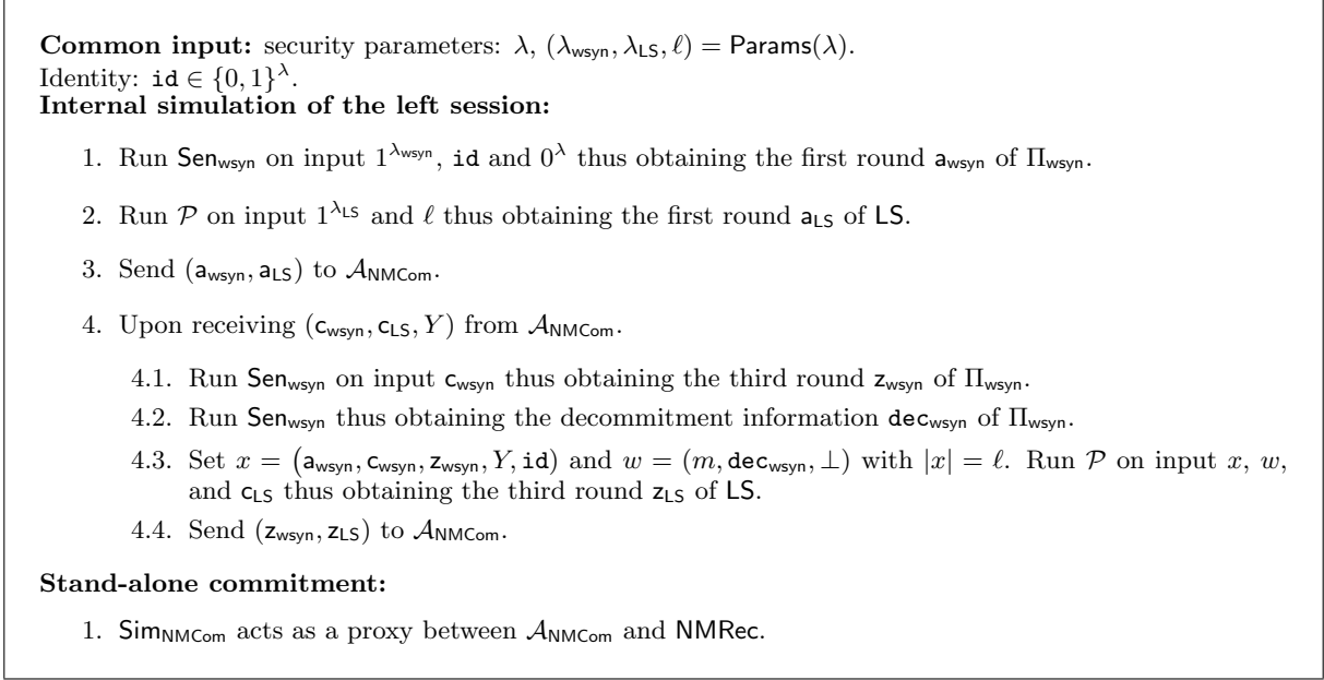
Figure 7: The simulator \text{Sim}_{\text{NMCom}} .
