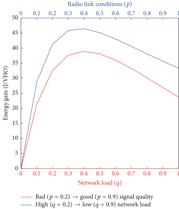
FIGURE 7: Effect of link and load conditions in the average energy consumption of the cooperation-assisted VHO mechanism.
