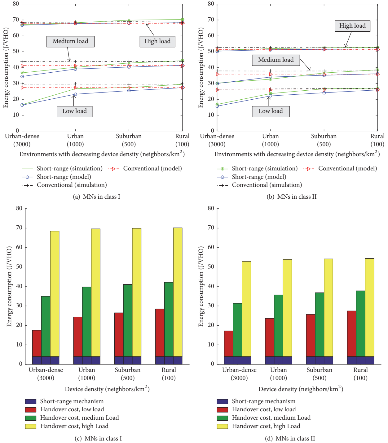
FIGURE 4: ((a) and (b)) Simulation and model-based average energy consumption of the cooperation-assisted VHO mechanism compared to that of the conventional VHO scheme for various network loads and device densities. ((c) and (d)) Energy breakdown of cooperation-assisted VHO mechanism.
