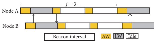
FIGURE 2: Modified periodically-fully-awake-interval protocol for the short-range cooperation between MNs. Neighbors exchange VHO-related information during AW and LW periods.
