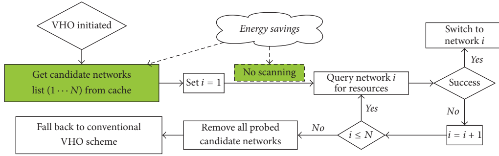
FIGURE 3: VHO procedure using the information obtained through the short-range cooperation mechanism.
