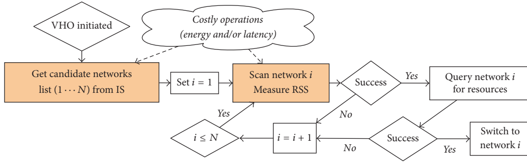
FIGURE 1: VHO procedure in the SCAN-FIRST scheme.
