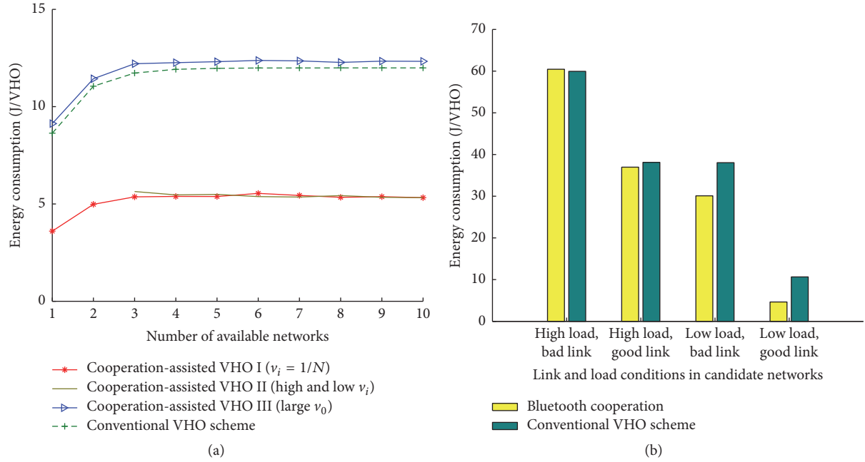
FIGURE 6: Average energy consumption of the cooperation-assisted VHO mechanism compared to that of the conventional VHO scheme in terms of the number of available networks and the network preference of the cooperating neighbors (a) and for various radio link and network load conditions (b).
