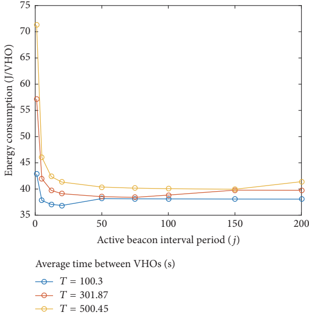
FIGURE 5: Impact of short-range cooperation mechanism configuration to the overall energy consumption.
