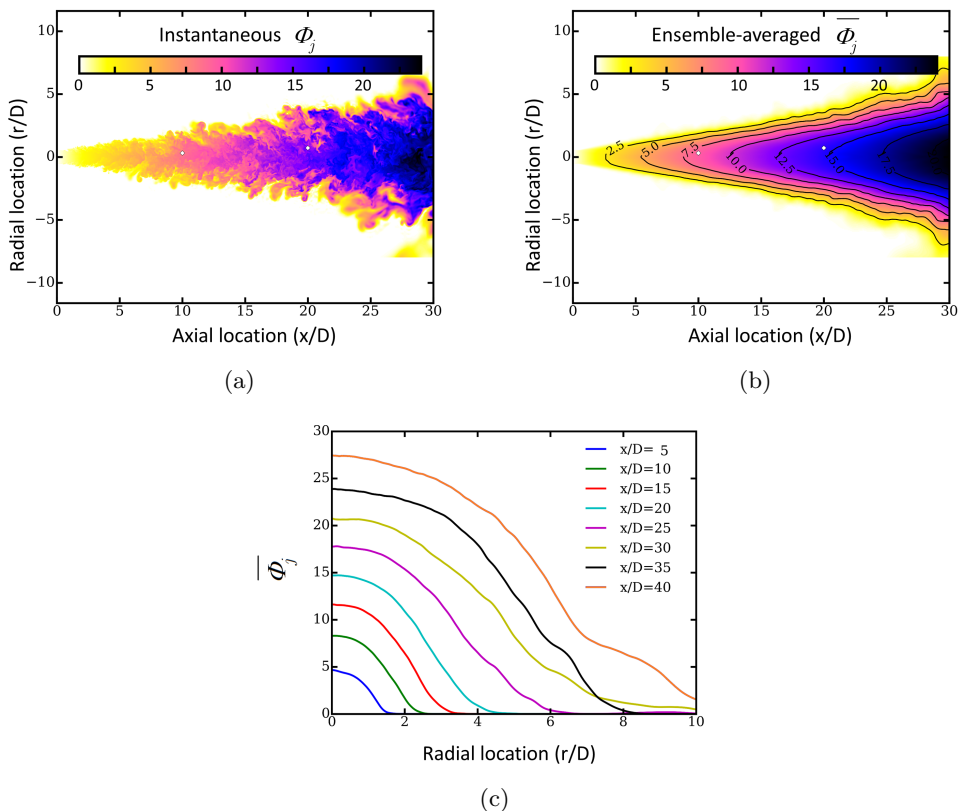
Figure 6: (a) Instantaneous mass-weighted stream age, \Phi_j and (b) ensemble-averaged \overline{\Phi_j} fields on a section through the jet centreline, and (c) the radial variation of \overline{\Phi_j} at different axial locations.
