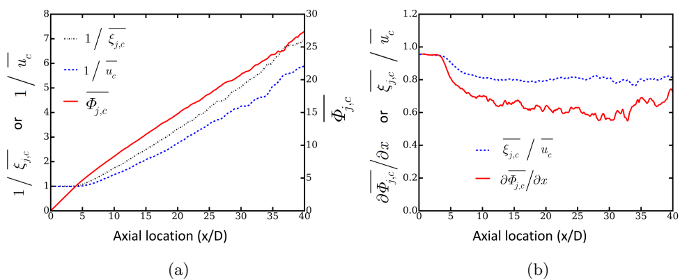
Figure 7: Axial variation of (a) the centreline average of mass-weighted stream age, \overline{\Phi_{j,c}} (right axis), the reciprocals of the centreline average mixture fraction 1/\overline{\xi_{j,c}} and axial velocity 1/\overline{u_c} (left axis). (b) The axial gradient of \overline{\Phi_{j,c}} and the ratio of \overline{\xi_{j,c}} and \overline{u_c} along the centreline.
