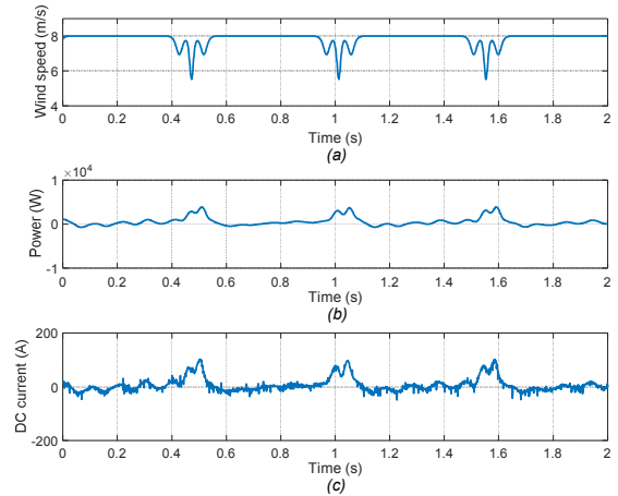
Fig. 11. Measurement results with lattice 45^\circ orientation tower shadow effect (a) modeled wind speed experienced by the blades (b) power difference between the generator and the load (point MA) (c) batteries DC current (point MB)
