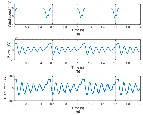
Fig. 10. Measurement results with lattice 22.5^\circ orientation tower shadow effect (a) modeled wind speed experienced by the blades (b) power difference between the generator and the load (point MA) (c) batteries DC current (point MB)
