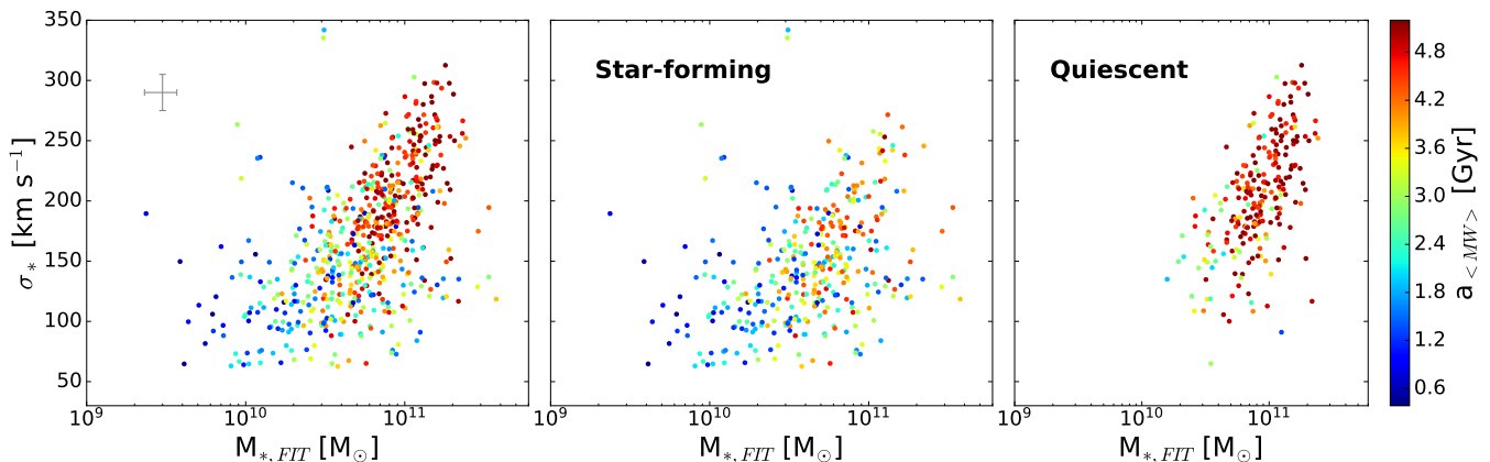
Figure 7. \sigma_* versus M_{*,FIT} , colour-coded by a_{<MW>} . The star-forming and quiescent populations are shown in the middle and right panels, respectively. Typical error bars are indicated in grey. The clear separation between young and old galaxies at \sigma_* \sim 170 \text{ km s}^{-1} shows a stronger correlation between a_{<MW>} and \sigma_* over M_{*,FIT} , which also depends on the current SF activity.
