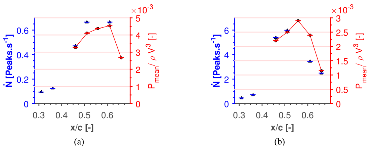
Figure 12. Mean values of aggressiveness intensity calculated at the hydrofoil chord – qualitative comparison with experimental results. ( \sigma\sim 1 , angle of attack: 4 deg.). (a) V=8\text{m/s} , (b) V=10.4\text{ m/s} . Comparative analyses concerns the real aggressive zone observed experimentally on the hydrofoil surface (i.e. x\geq 0.4c ).
