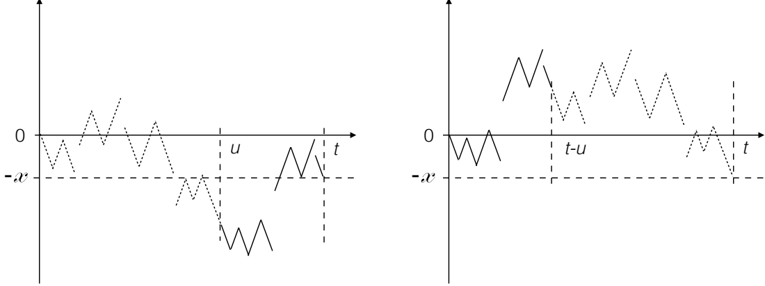
A path \omega of \mathcal{D}_t on the left and the shifted path \theta_u(\omega) on the right.
