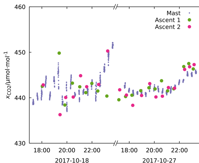
Figure 12. Large dots represent calibrated measurements taken by COCAP during the ascents at a height of (40 \pm 10) \text{ m} above ground, small dots are measurements from the LIN mast’s 40 m inlet. Times are in local time (UTC+2). The sun set at 18:02 LT on 18 October and at 17:43 LT on 27 October. The gaps in the station data are due to the measurement of other inlets and working tanks at those times.
