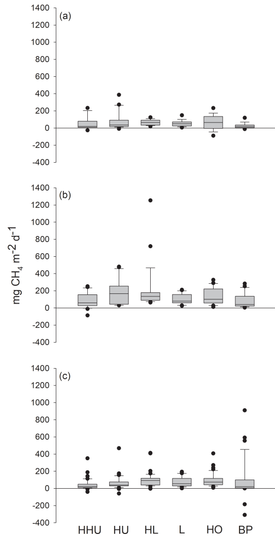
Figure 2. Methane fluxes in the Siikaneva bog in the three subsequent years (a) 2012, (b) 2013 and (c) 2014 from six different plant community types: high hummock (HHU), hummock (HU), high lawn (HL), lawn (L), hollow (HO) and bare peat surfaces (BP).
