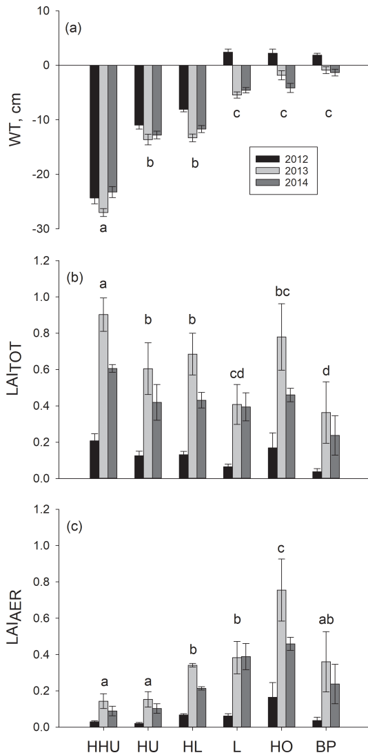
Figure 1. (a) Mean water table and the mean of summer maximum of (b) total leaf area (LAI TOT ) and (c) leaf area of aerenchymatous plant species (LAI AER ) in six plant community types: high hummock (HHU), hummock (HU), high lawn (HL), lawn (L), hollow (HO) and bare peat surface (BP) in three subsequent years. The error bars show the standard error of the mean. The different letters (a–d) denote significant differences between the plant community types. The same letter above bars indicates that those plant community types do not differ statistically from each other. Note: statistical analyses for LAI have been conducted with mean LAI TOT and LAI AER instead of summer maximum.
