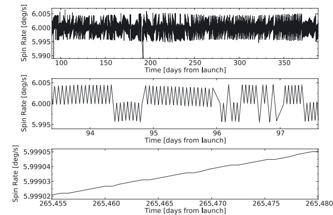
Fig. 9. The top panel shows the measured spin rate over the coverage period, which is always within \pm 0.1\% of 1 rpm. The spin rate typically adopts one of three values as can be seen in the middle panel, which is a zoom into a period of several days. In the bottom panel we show the typical drift of the spin rate within a dwell, due to small residual torques applied to the satellite.
