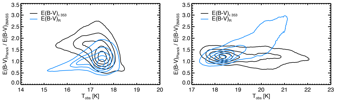
Fig. 25. Two-dimensional histogram of E(B - V)_{\tau_{353}}/E(B - V)_{2MASS} (black contours) and E(B - V)_{\mathcal{R}}/E(B - V)_{2MASS} (blue contours) as a function of T_{obs} , for the Taurus ( left ) and \rho Ophiuchi ( right ) molecular clouds. The maps used are those shown in Figs. 23 and 24.
