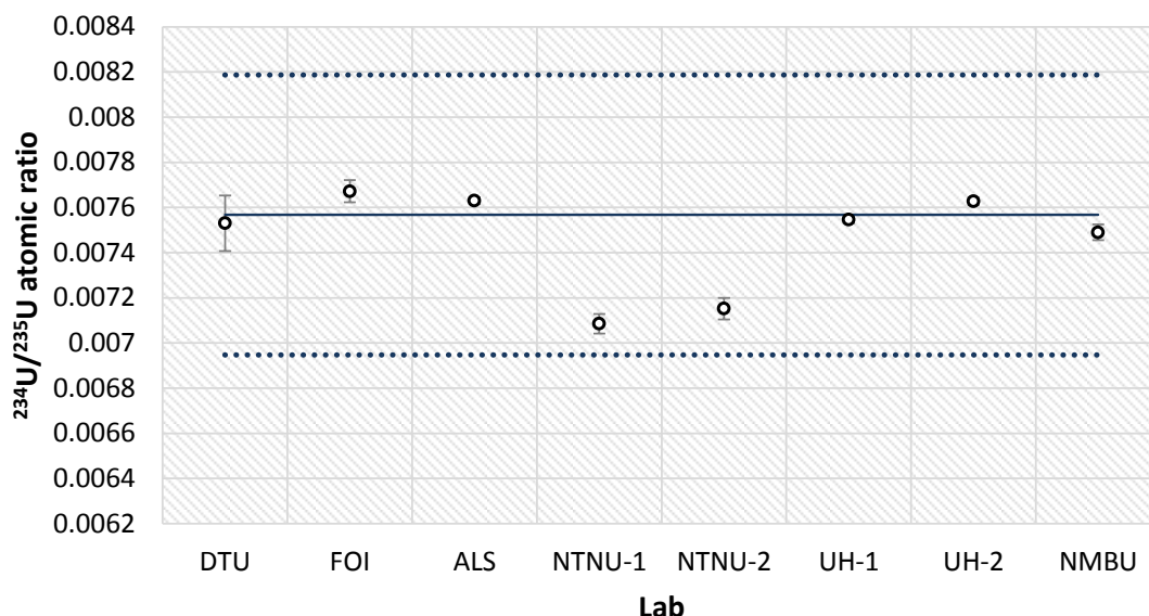
Figure 1 ^{234}\text{U}/^{235}\text{U} isotope ratios from the measurement of the reference material NBL CRM 103-A. The solid and dotted lines represent the observed average and variation of natural uranium, respectively 10 . The error bars of the results represent the expanded uncertainty with a coverage factor, k=1 .
