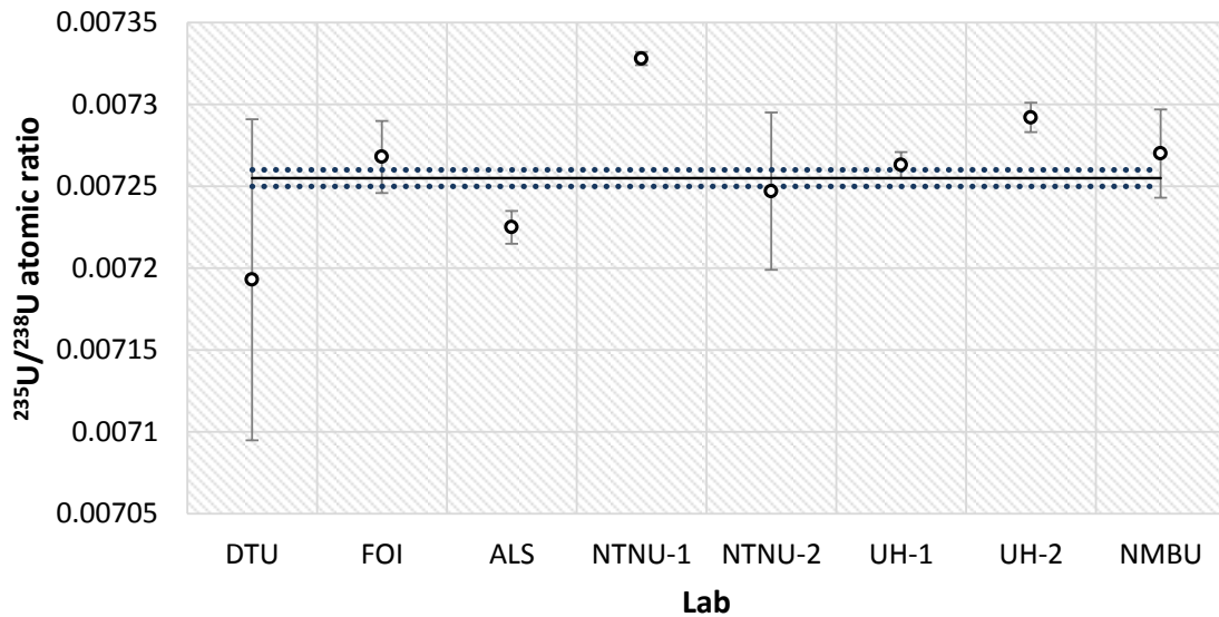
Figure 3 ^{235}\text{U}/^{238}\text{U} isotope ratios from the measurement of the reference material NBL CRM 103-A. The solid and dotted lines represent the observed average and variation of natural uranium, respectively 10 . The error bars of the results represent the expanded uncertainty with a coverage factor, k=1 .
