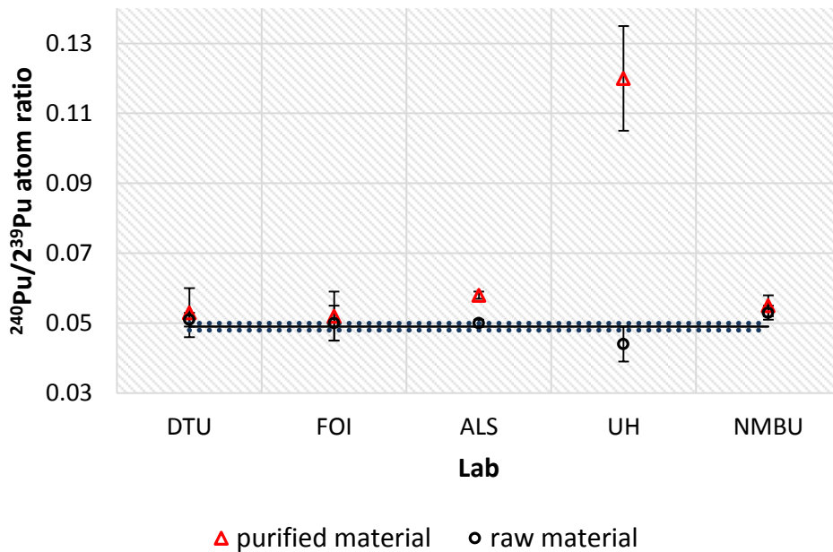
Figure 13 ^{240}\text{Pu}/^{239}\text{Pu} atomic ratio from the measurement of the reference material IAEA-384. The solid line represents the reference value and dotted lines represent the 95% confidential interval (Povinec et al, 2007). The error bars of the results represent the expanded uncertainty with a coverage factor, k=1 .
