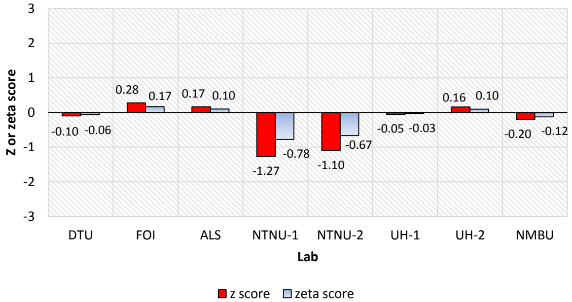
Figure 2 Z-score and zeta -score calculated for ^{234}\text{U}/^{235}\text{U} atomic ratios from the measurement of the reference material NBL CRM 103-A.
