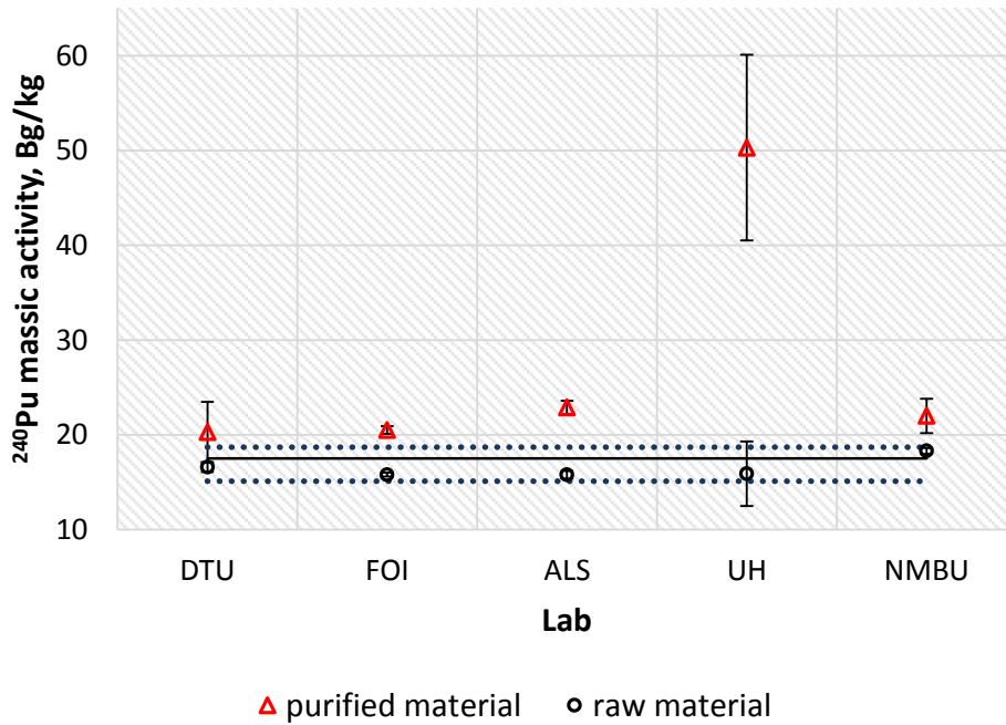
Figure 10 ^{240}\text{Pu} massic activities from the measurement of the reference material IAEA-384. The solid line represents the reference value and dotted lines represent the 95% confidential interval 11 . The error bars of the results represent the expanded uncertainty with a coverage factor, k=1 .
