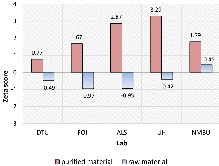
Figure 12 Zeta-score calculated for ^{240}\text{Pu} massic activity from the measurement of the reference material IAEA-384.
