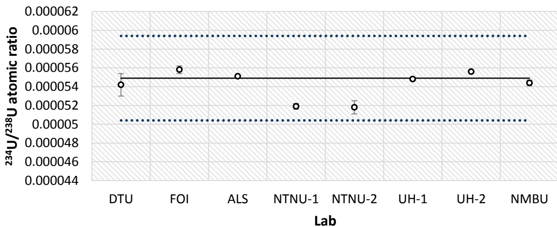
Figure 5 ^{234}\text{U}/^{238}\text{U} isotope ratios from the measurement of the reference material NBL CRM 103-A. The solid and dotted lines represent the observed average and variation of natural uranium, respectively 10 . The error bars of the results represent the expanded uncertainty with a coverage factor, k=1 .
