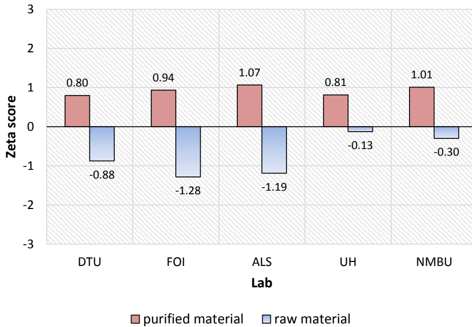
Figure 9 Zeta-score calculated for ^{239}\text{Pu} massic activity from the measurement of the reference material IAEA-384.
