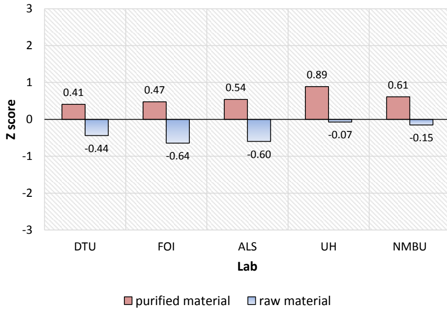
Figure 8 Z-score calculated for ^{239}\text{Pu} massic activity from the measurement of the reference material IAEA-384.
