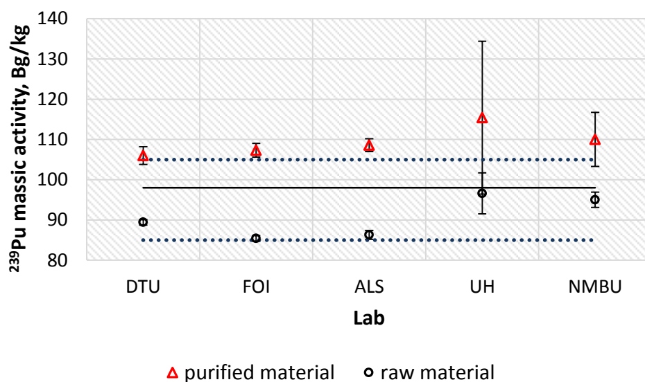
Figure 7 ^{239}\text{Pu} massic activities from the measurement of the reference material IAEA-384. The solid line represents the reference value and dotted lines represent the 95% confidential interval 11 . The error bars of the results represent the expanded uncertainty with a coverage factor, k=1 .
