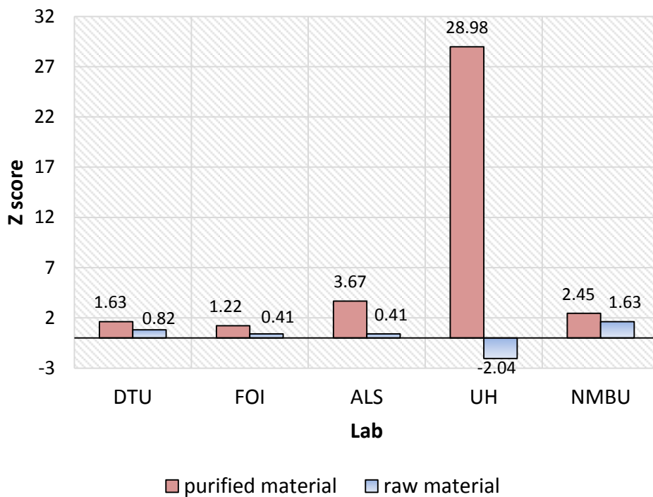
Figure 14 Z-score calculated for ^{240}\text{Pu}/^{239}\text{Pu} atomic ratios from the measurement of the reference material NBL IAEA-384.
