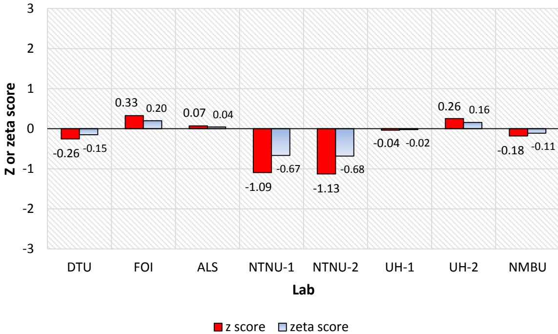
Figure 6 Z-score and zeta -score calculated for ^{234}\text{U}/^{238}\text{U} atomic ratios from the measurement of the reference material NBL CRM 103-A.
