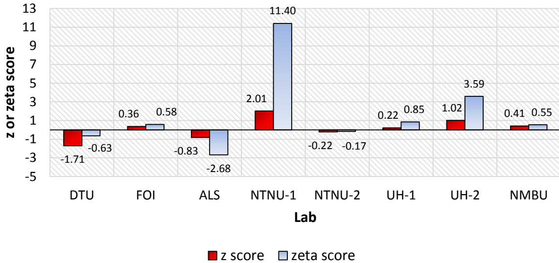
Figure 4 Z-score and zeta -score calculated for ^{235}\text{U}/^{238}\text{U} atomic ratios from the measurement of the reference material NBL CRM 103-A.
