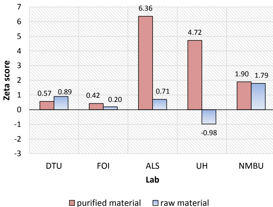
Figure 15 Zeta-score calculated for ^{240}\text{Pu}/^{239}\text{Pu} atomic ratios from the measurement of the reference material NBL IAEA-384.
