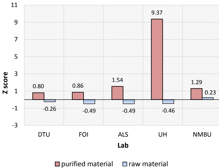
Figure 11 Z-score calculated for ^{240}\text{Pu} massic activity from the measurement of the reference material IAEA-384.
