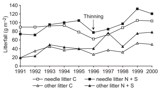
Fig. 2. Annual litterfall of the Scots pine stand during 1991–2000. C = control treatment, N + S = annual application of ammonium sulphate.
