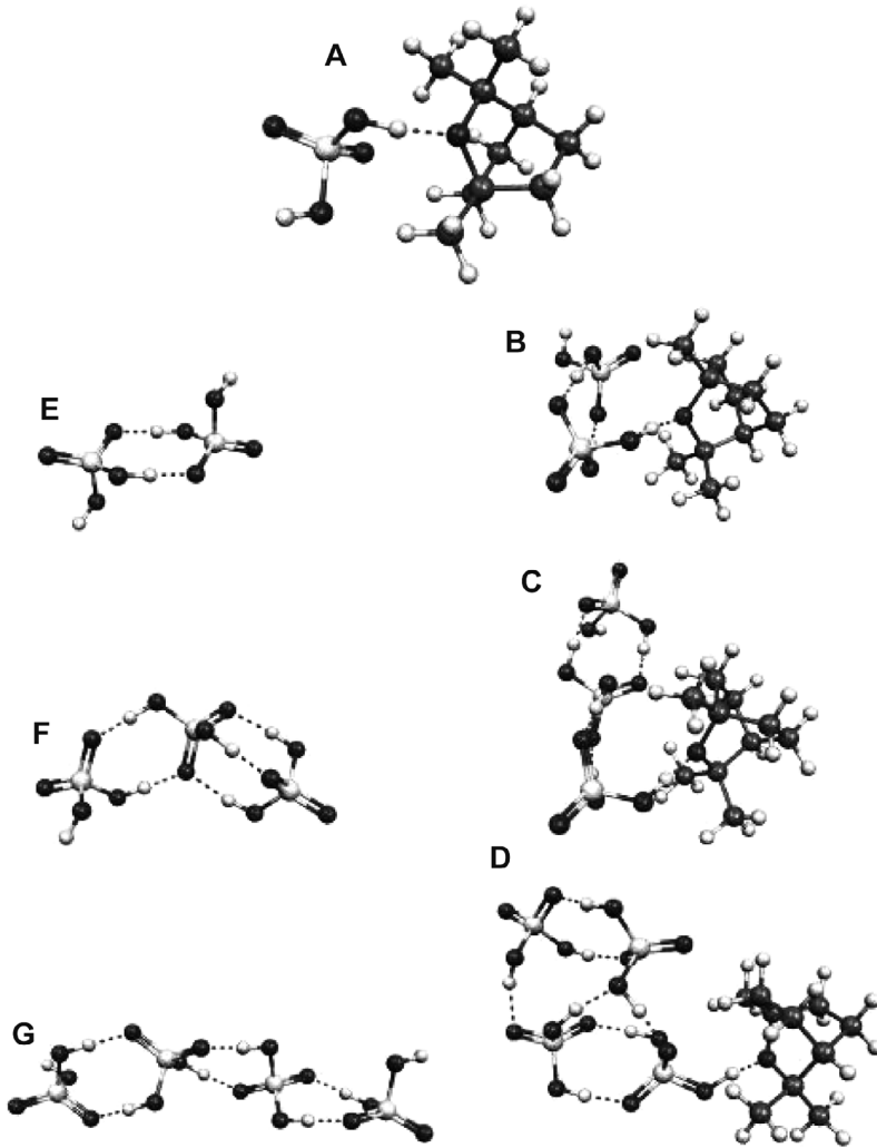
Fig. 5. Structures of the most stable cluster configurations obtained with the SIESTA model. A , B , C and D represent clusters with one molecule of eucalyptol and one to four molecules of sulfuric acid, respectively. E , F and G represent clusters containing from two to four sulfuric acid molecules, respectively. Black atoms correspond to oxygen, light grey to sulfur, dark grey to carbon and white to hydrogen.
