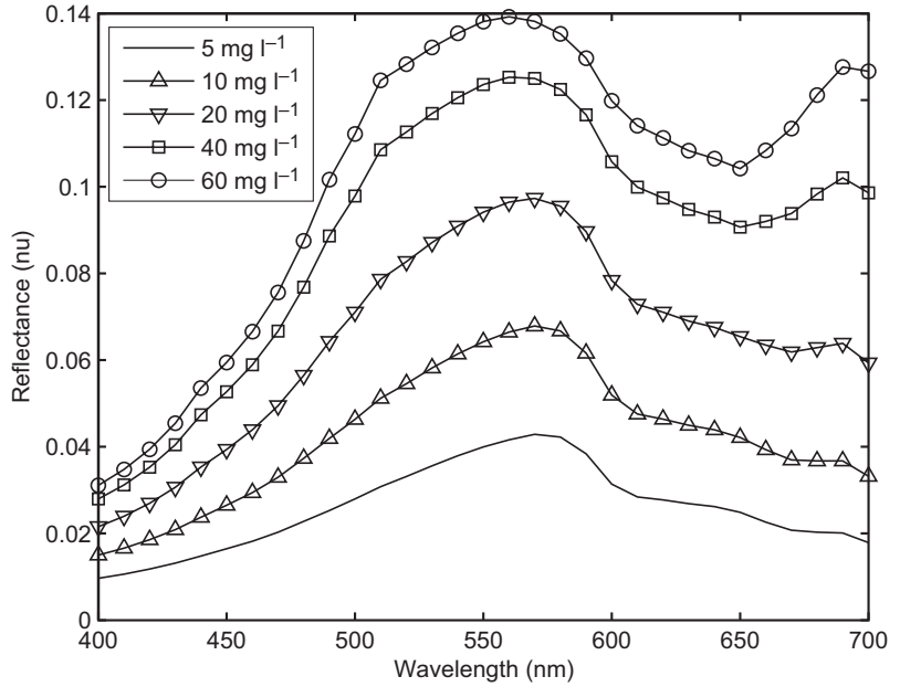
Fig. 3. Modelled surface reflectances with varying C_{SM} ( mg\ l^{-1} ) concentrations.
