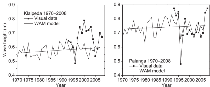
Fig. 5. Modelled and visually observed annual mean wave heights on the SE coast of the Baltic Sea. Modelled data were kindly provided by Dr. A. Räämet.
