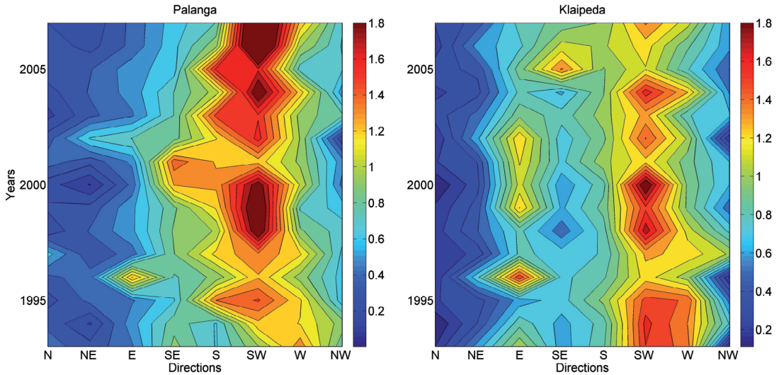
Fig. 8. Temporal course of the frequency of waves from different directions in 1993–2007 at Klaipėda and Palanga. The color scale shows the frequency of occurrence (%) of different wave propagation directions.
