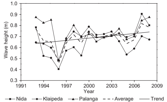
Fig. 4. Annual mean wave heights on the SE coast of the Baltic Sea. The linear trend is calculated for the average over all three sites. Modified from Kelpšaitė et al. (2008), with permission from the Estonian Academy Publishers.
