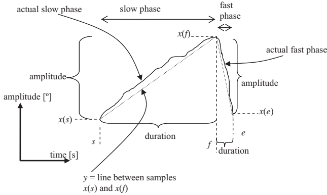
Fig. 2 A hypothetical nystagmic beat describing its main variables and shape from which some other variables are derived. A beat is composed of the slow and fast phases represented with their amplitudes given in angular degrees and durations in seconds. In reality, there may be noise or other unevenness in nystagmus signals. Such phenomena are estimated by computing, for example, linear correlation between an actual slow phase and its ideal component, straight line y .
