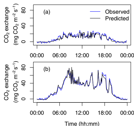
Figure 2. Measured and predicted leaf \text{CO}_2 exchange during 2 days: (a) early in the spring (8 May) and (b) in midsummer (18 July) in Finnish Lapland, 68^\circ\text{N} .
