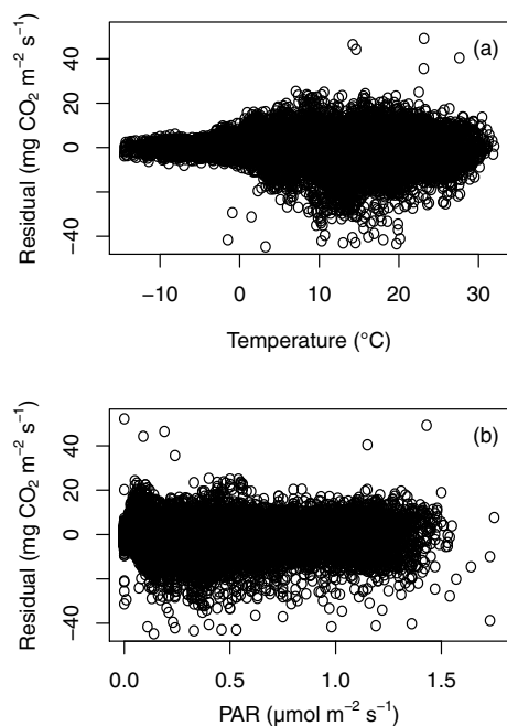
Figure 5. The residuals as a function of temperature and PAR in the year 2013 in Finnish Lapland, 68° N.
