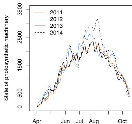
Figure 1. The annual pattern of the state of the photosynthetic machinery ( S , arbitrary units) during the years 2011–2014 in Finnish Lapland, 68^\circ\text{N} .
