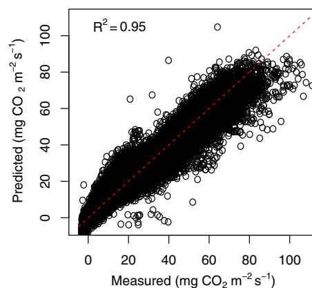
Figure 4. Relationship between the measured and predicted leaf \text{CO}_2 exchange in Finnish Lapland, 68^\circ \text{N} in the year 2013. The dashed line represents the 1 : 1 line.
