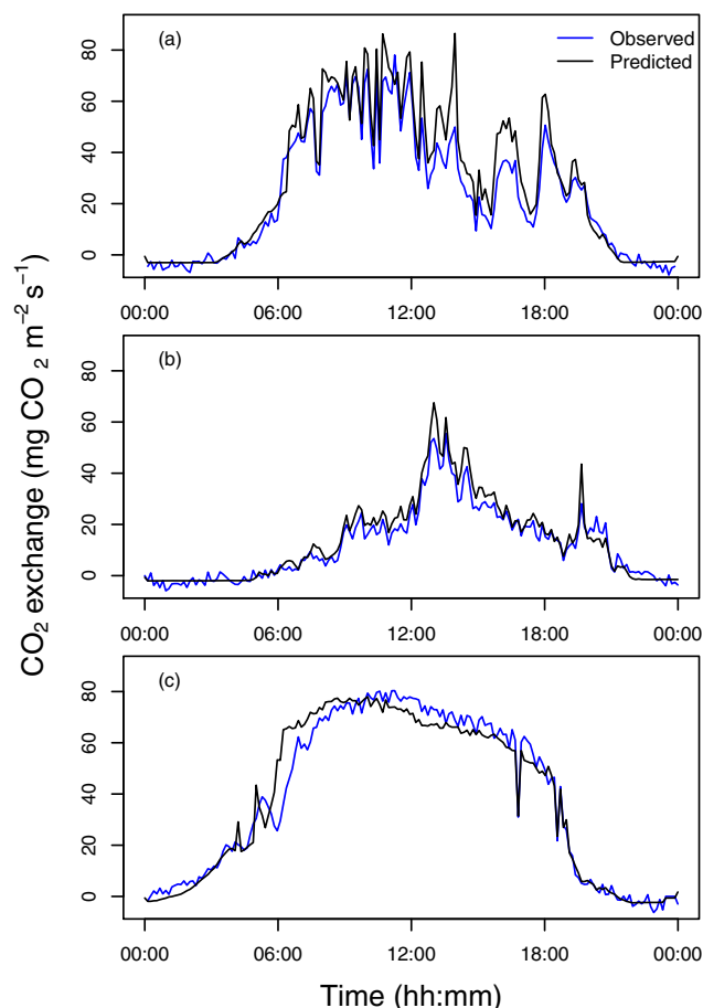
Figure 3. Measured and predicted leaf \text{CO}_2 exchange (a) during a day of intermittent cloudiness (5 August), (b) during a cloudy day (22 July), and (c) during a sunny day when the stomata close partially (7 July) in Finnish Lapland, 68^\circ \text{N} .
