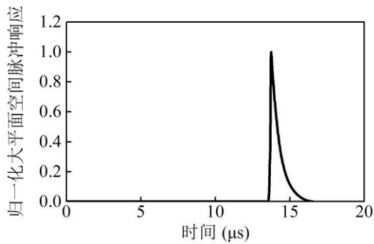
Fig.4 The impulse response of the plane test block. Fig.5 The response of the plane test block
