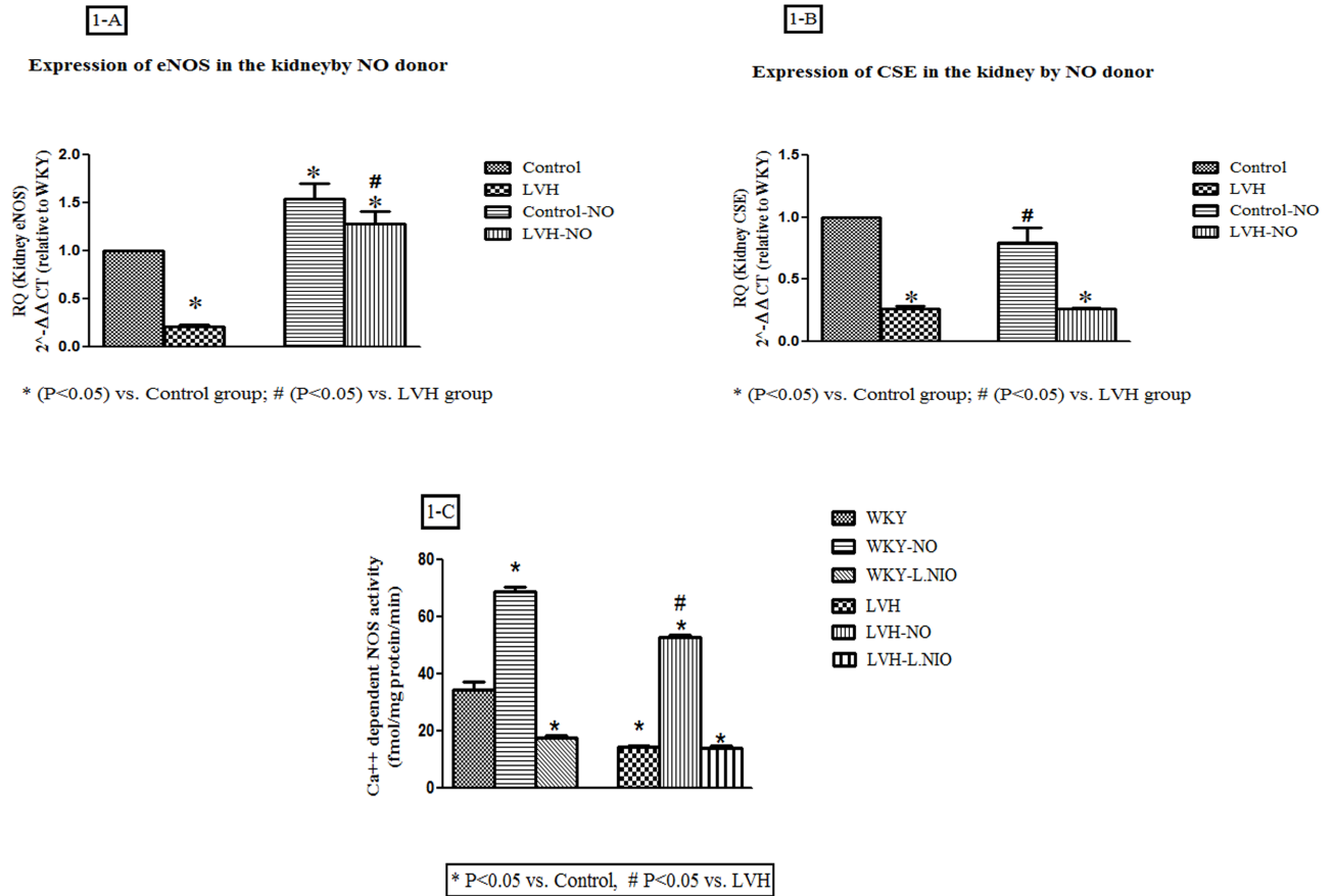
Fig 1. A, B, C) showing the molecular expression of CSE and eNOS mRNAs and NOS activity in the cortex of kidney of the Control, LVH, Control-NO and LVH-NO rats. Data is shown as \pm SEM while significance is taken as p < 0.05 .
