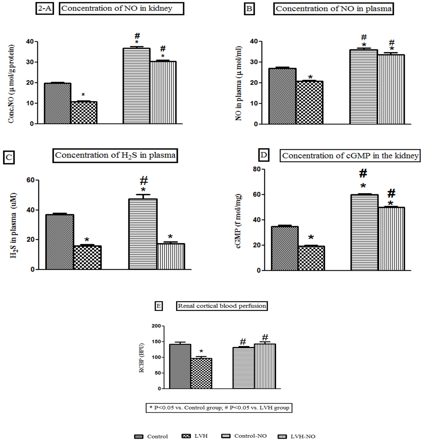
Fig 2. Showing the concentration of nitric oxide in the kidney (A), nitric oxide in plasma (B), H 2 S in plasma (C), cGMP in the kidney (D) and renal cortical blood perfusion of Control, LVH, Control-NO and LVH-NO rats. Data is shown as \pm SEM while significance is taken as p < 0.05 . * ( P < 0.05 ) vs. Control group; # ( P < 0.05 ) vs. LVH group.
