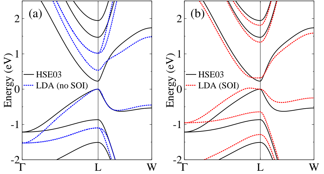
Figure 5.15: Electronic bands for PbTe calculated using the HSE03 functional including SOI (solid black lines) compared with those calculated using the LDA functional (a) excluding SOI (dashed blue lines) and (b) including SOI (dashed red lines).
