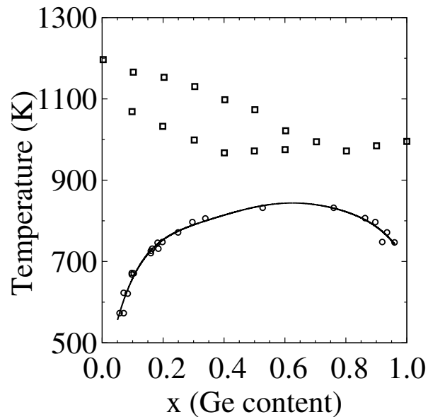
Figure 4.33: The quasi-binary phase diagram of \text{Pb}_{1-x}\text{Ge}_x\text{Te} alloys, reproduced from experimental data from Ref. [157] and references therein. The miscibility gap is shown with black circles, the liquidus and solidus temperatures are shown in black squares for each alloy composition.
