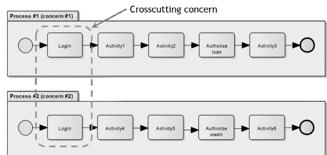
Fig. 1. Tangled and scattered crosscutting concern.
