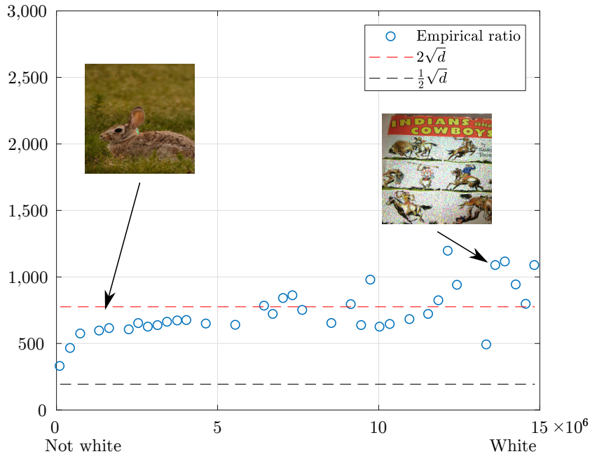
Figure 9: Fraction \frac{r_{\Sigma(\mathbf{x}),\varepsilon}(\mathbf{x})}{\|\mathbf{r}_2^*(\mathbf{x})\|_2} , where \varepsilon = 15\% , as a function of W(\mathbf{x}) . W(\mathbf{x}) encodes how “white” the pixels of the image are. Under our noise model, images with small W(\mathbf{x}) will have the noise concentrated along a few pixels, while images with large W(\mathbf{x}) will have their noise spread across most pixels in the image. Each circle represents the average robustness ratio of images with the same W(\mathbf{x}) .
