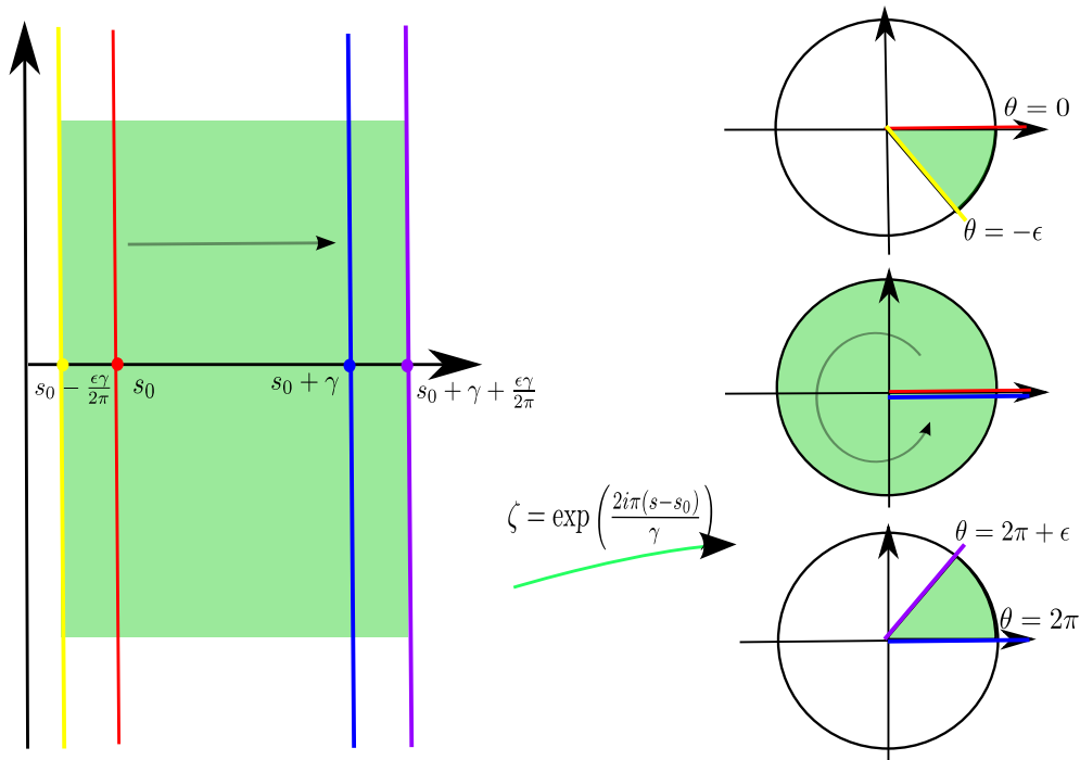
Figure 1: Holomorphic change of coordinates sends the green strip s_0 - \frac{\epsilon\gamma}{2\pi} < \Re(s) < s_0 + \gamma + \frac{\epsilon\gamma}{2\pi} (Left) into the green subdomain D(\epsilon) (Right) of the Riemann surface associated to the logarithmic function.
