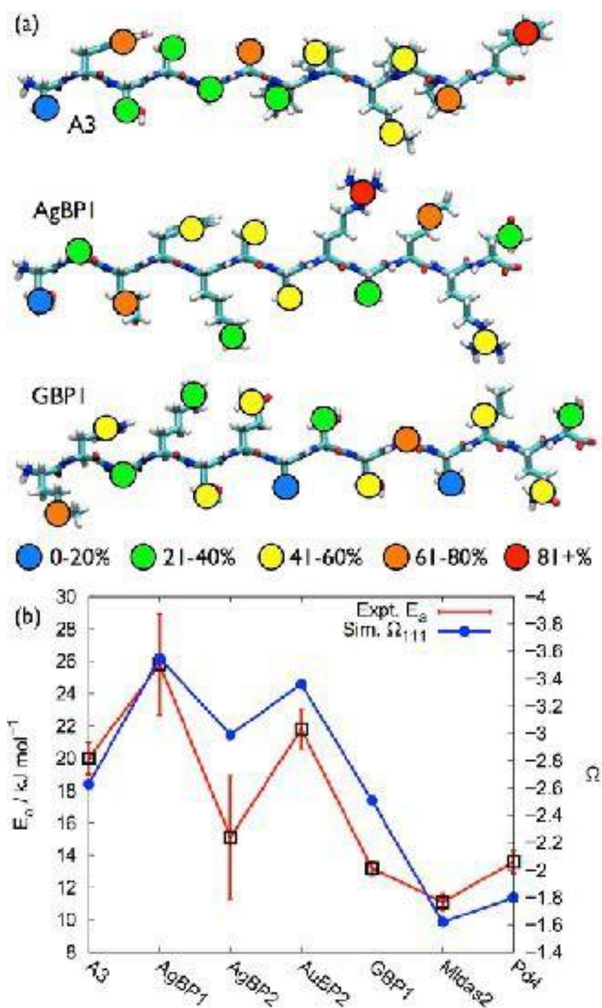
Figure 5. (a) Average degree of residue Au NP surface contact, indicated by the colored circles, for the A3, AgBP1, and GBP1 peptides. (b) The relationship between the activation energies and the contact score on the Au(111) for peptides at least 12 residues in length.
