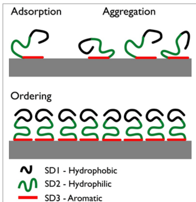
Figure 1: Illustration of the three stages of the previously-proposed surface-induced organization mechanism of GrBP5-WT.9 Initial surface contact proceeds via aromatic residues in SD3. As surface coverage increases, the peptide chains form a disordered surface-adsorbed aggregate. Ultimately, the coverage reaches a critical threshold and the chains self-organize into an ordered over-layer via inter-chain interactions of SD1.
