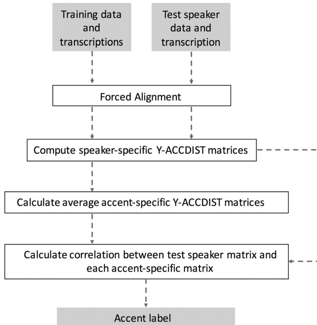
FIG. 2. Y-ACCDIST system flow diagram.
