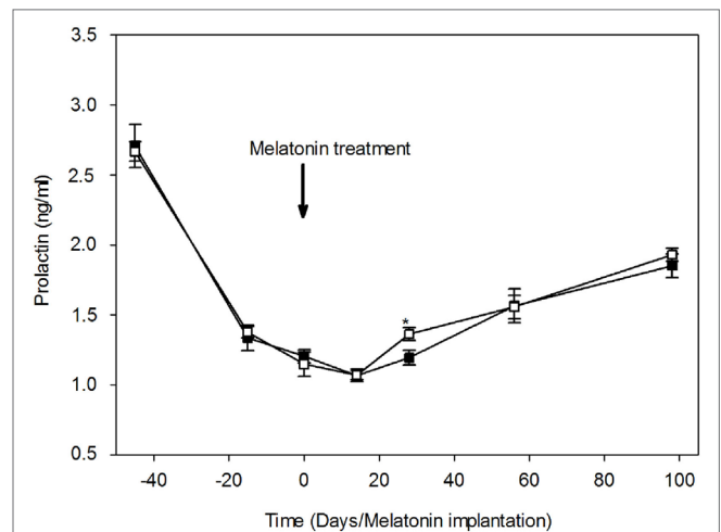
FIGURE 4 | Variations of plasma prolactin concentrations (mean \pm SEM) in camel females of the melatonin-treated group (■) and control group (□). Time is expressed as days relative to the melatonin implants insertion: before and after day 0. At day 28, prolactin concentration was significantly (* P < 0.05 ) lower in the melatonin-treated group compared to the control group.
