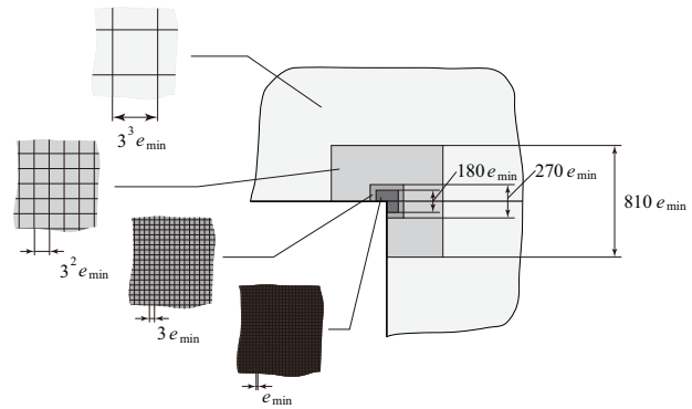
Figure 7. Mesh pattern near the interface end.
